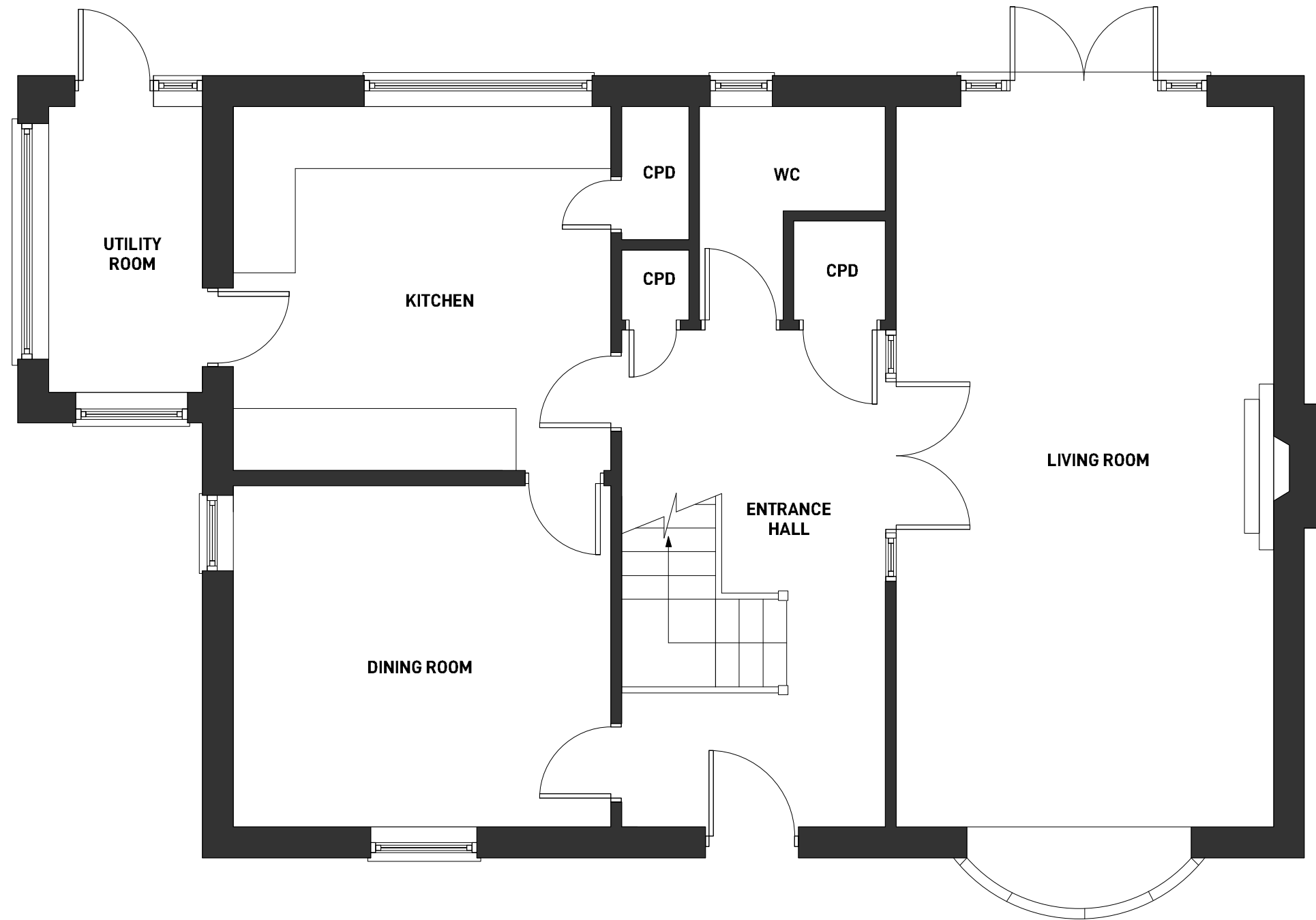
1 EXISTING GROUND FLOOR PLAN 01 SCALE 1:50 @A3
