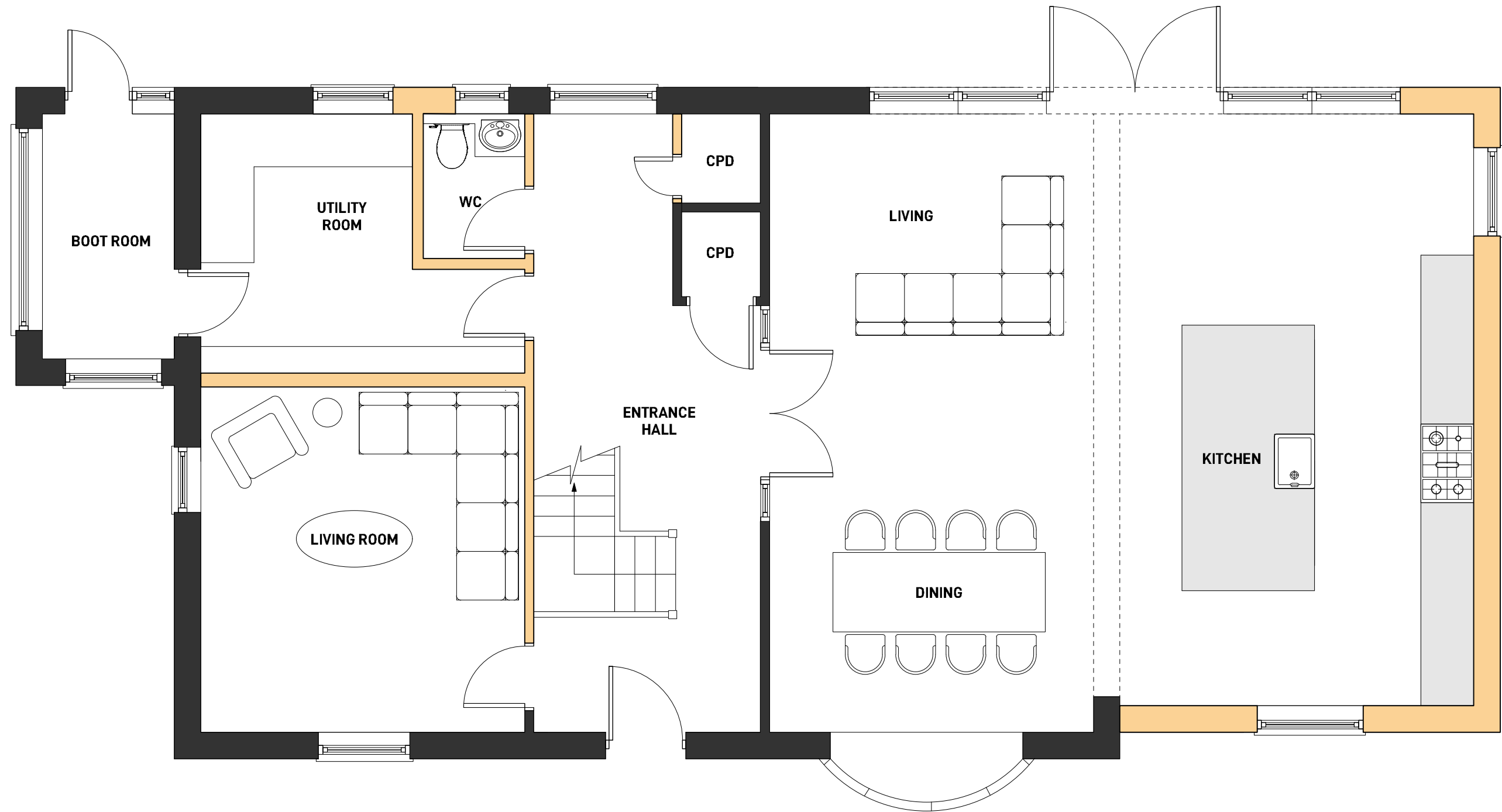
1 PROPOSED GROUND FLOOR 05 SCALE 1:50 @A3
