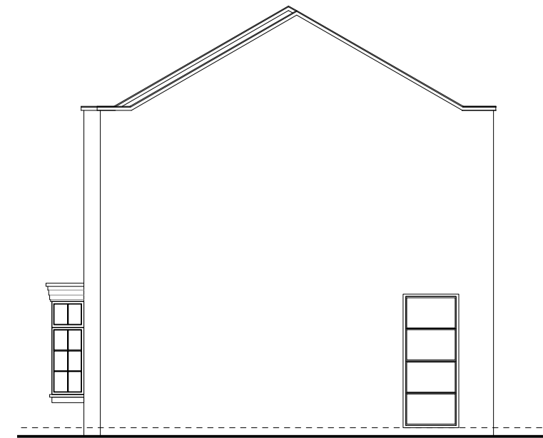
2 PROPOSED SIDE ELEVATION 07 SCALE 1:100 @A3
