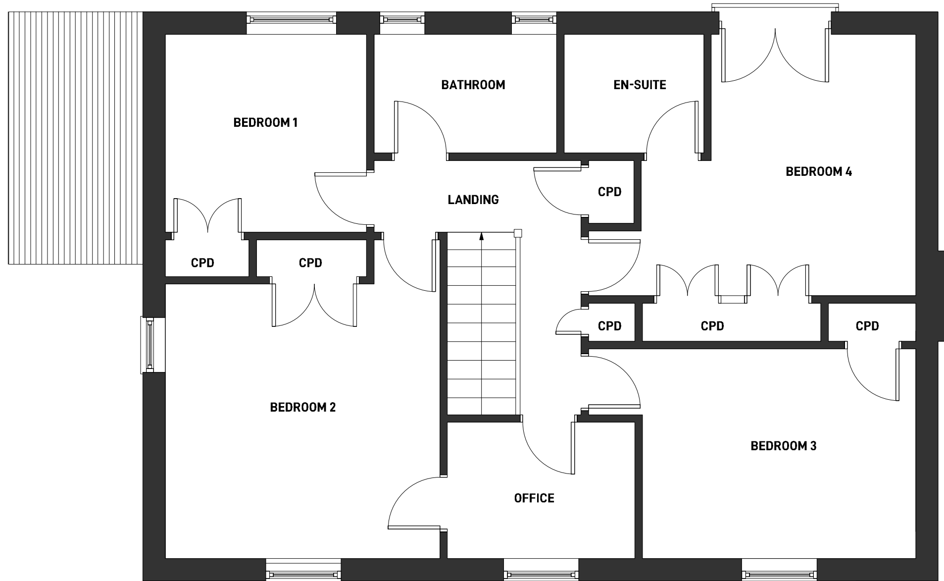
1 EXISTING FIRST FLOOR PLAN 02 SCALE 1:50 @A3
