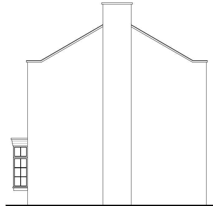
2 EXISTING SIDE ELEVATION 08 SCALE 1:100 @A3
