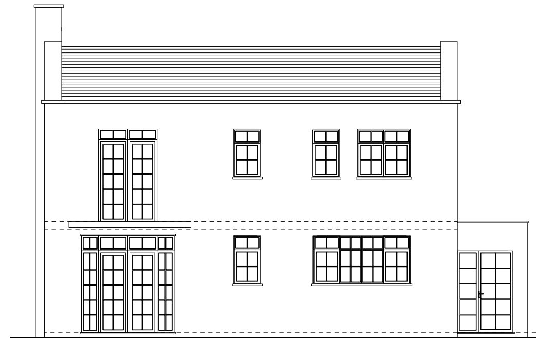
4 EXISTING REAR ELEVATION 08 SCALE 1:100 @A3
