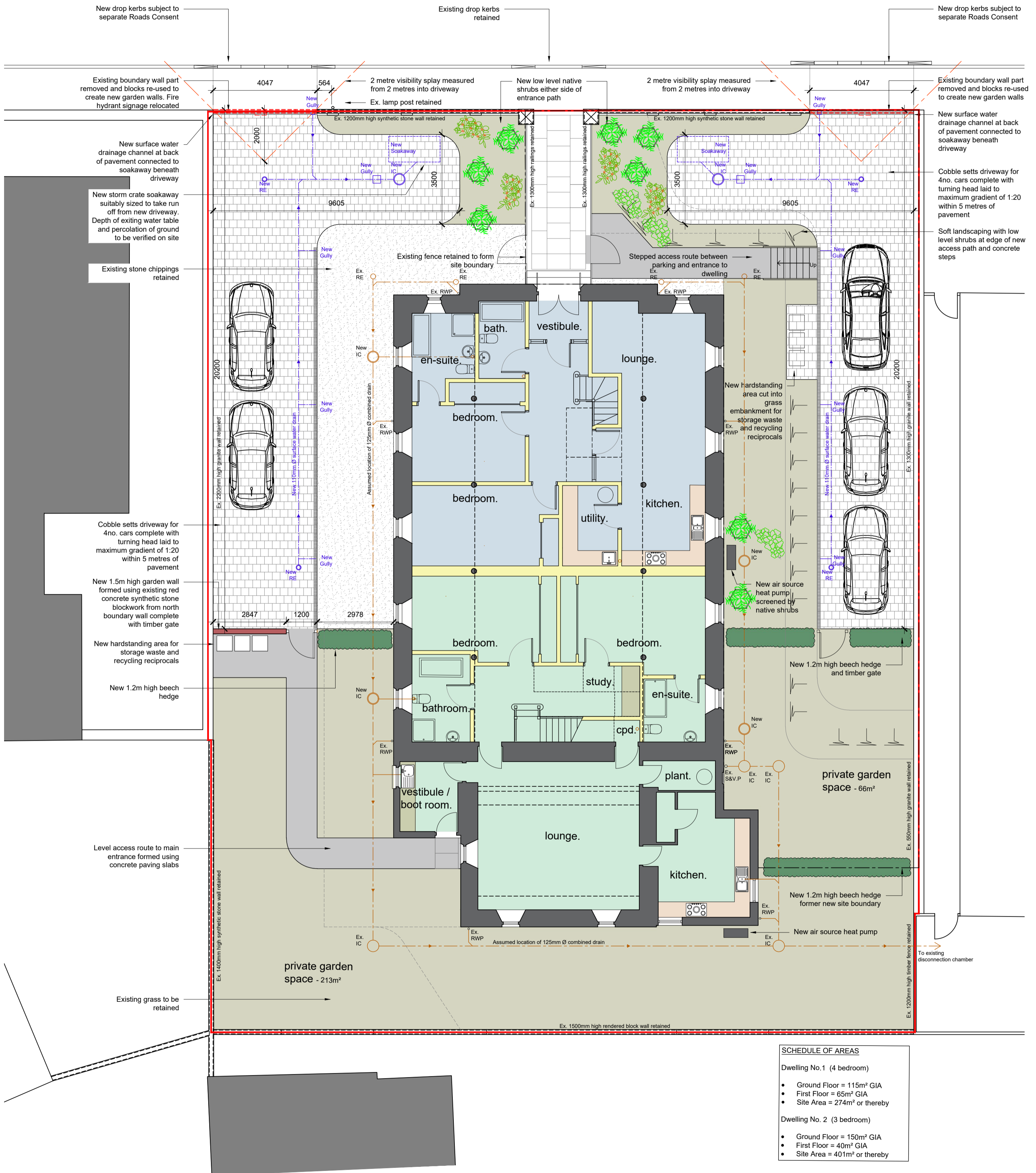
PROPOSED SITE LAYOUT PLAN - 1:100
