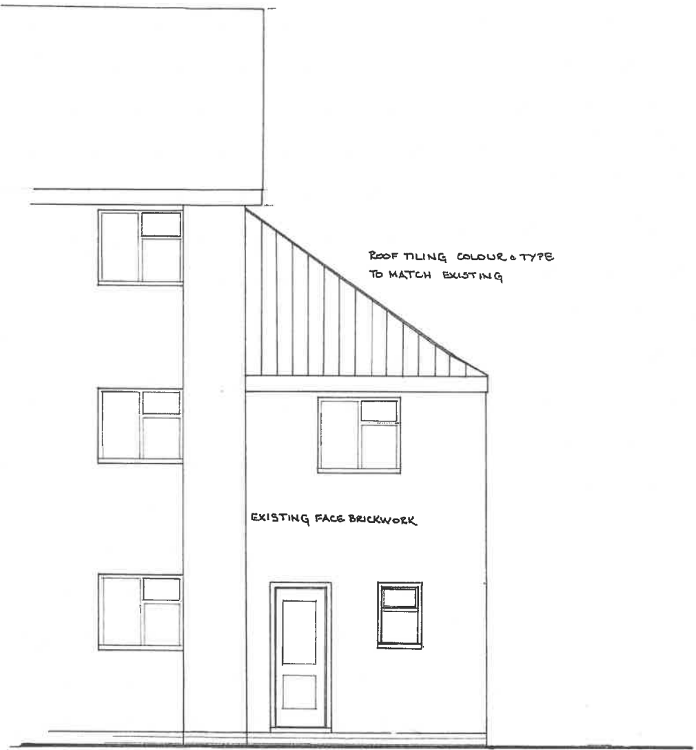
EXISTING REAR ELEVATION SCALE 1:50
