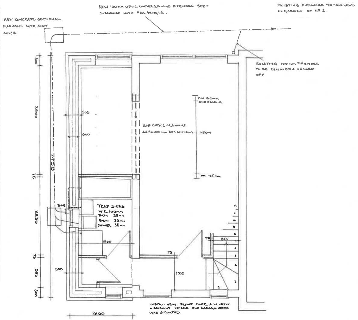
PROPOSED GROUND & FIRST FLOOR PLANS DETAILS
