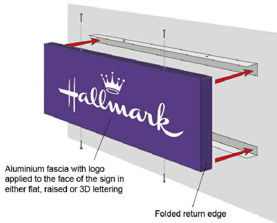
TYPICAL FIXING DETAILS (NTS)
