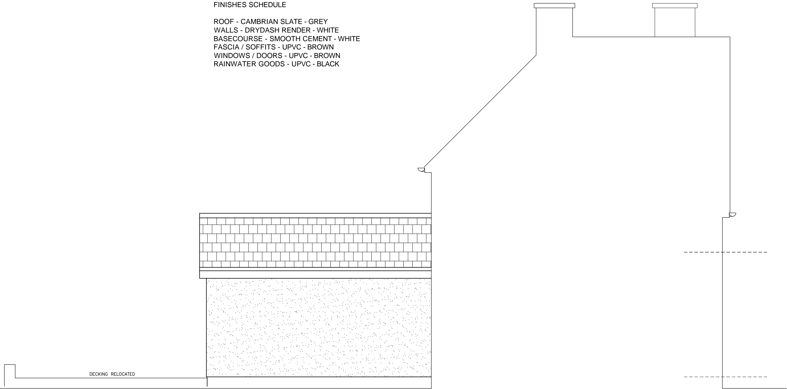
SECTIONAL ELEVATION AS PROPOSED
