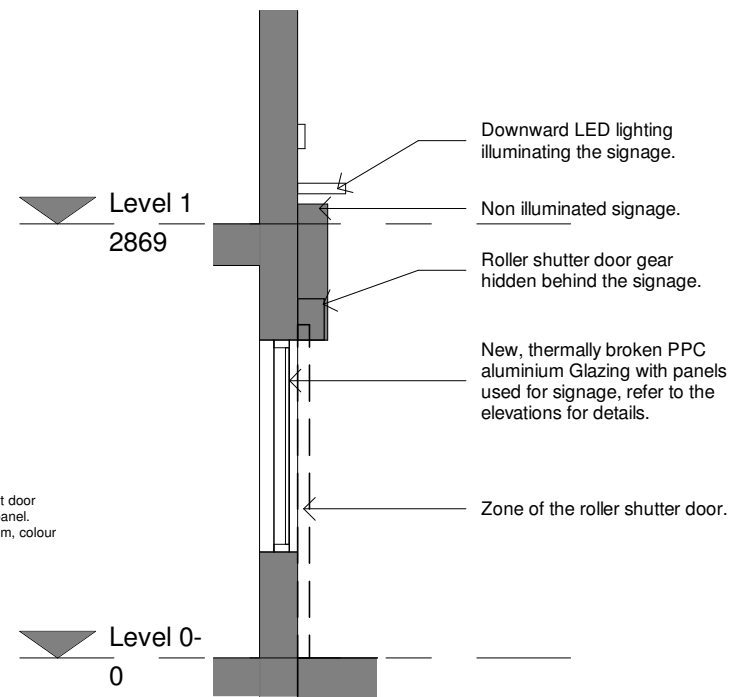
05 | Section thru the gazed frontage 1 : 50
