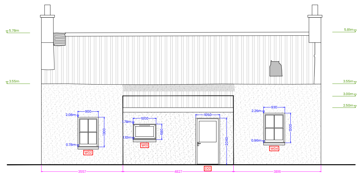
East Elevation - Existing 1:100
