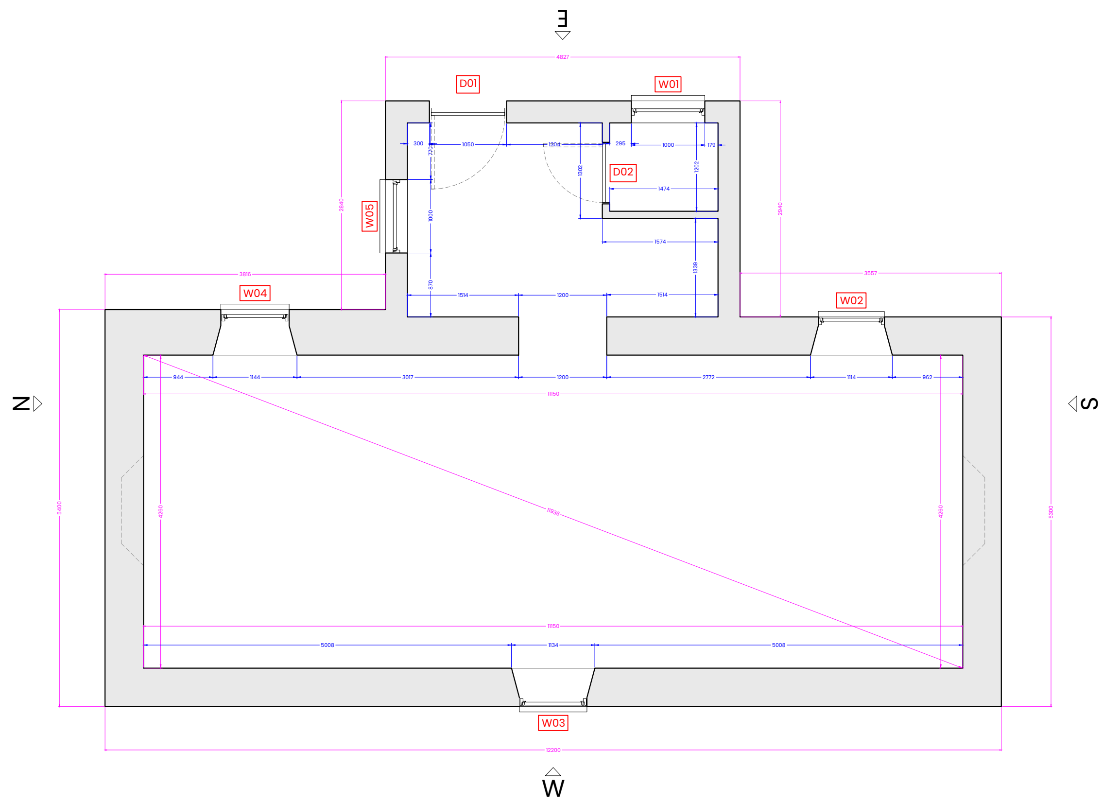
Floor Plan - Existing 1:50
