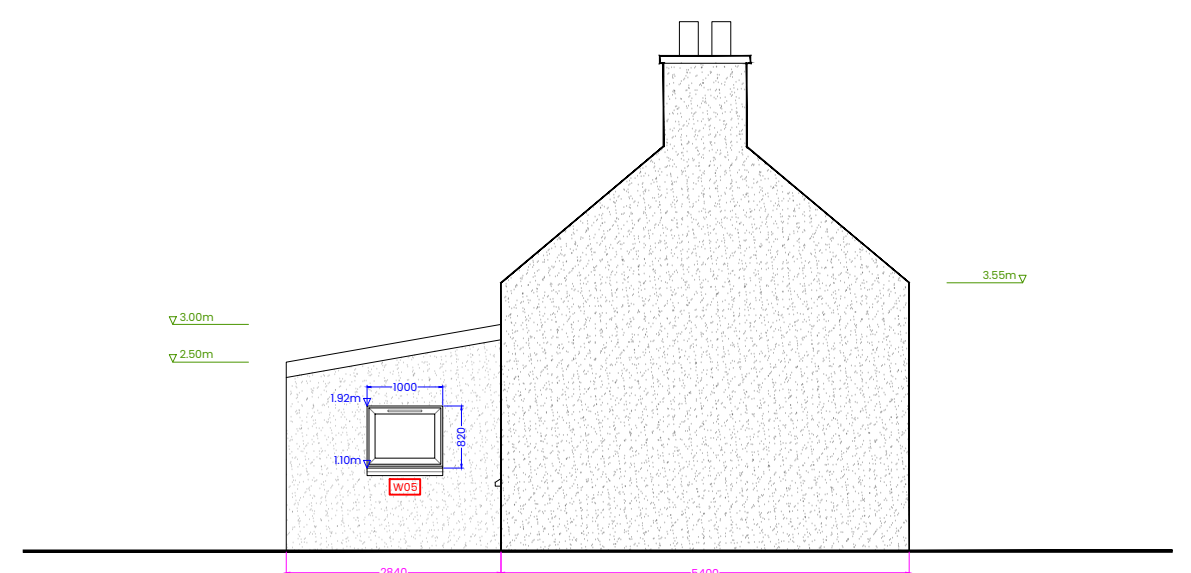
North Elevation - Existing 1:100
