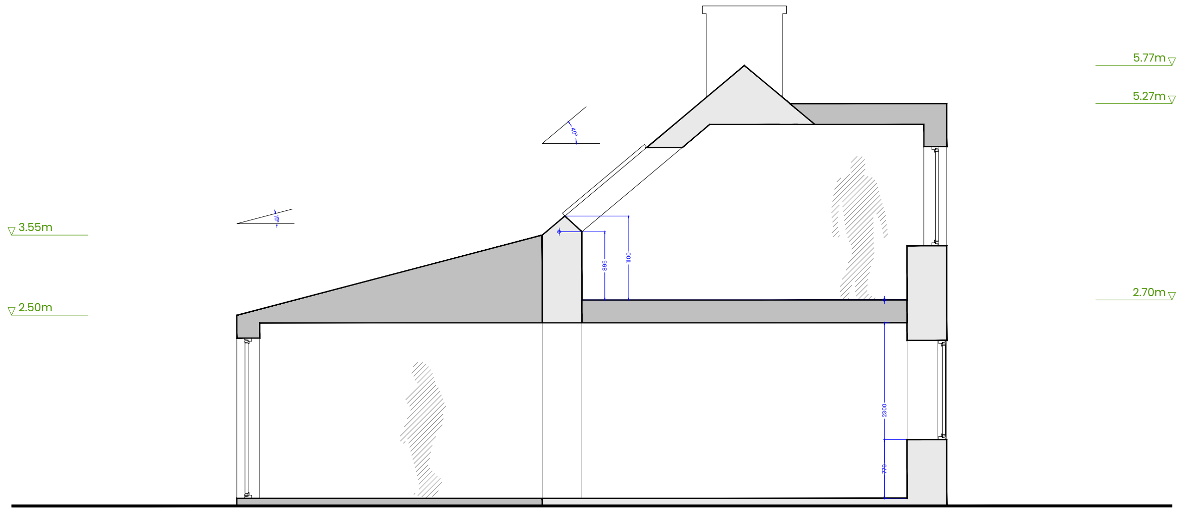
Section - Proposed 1:50
