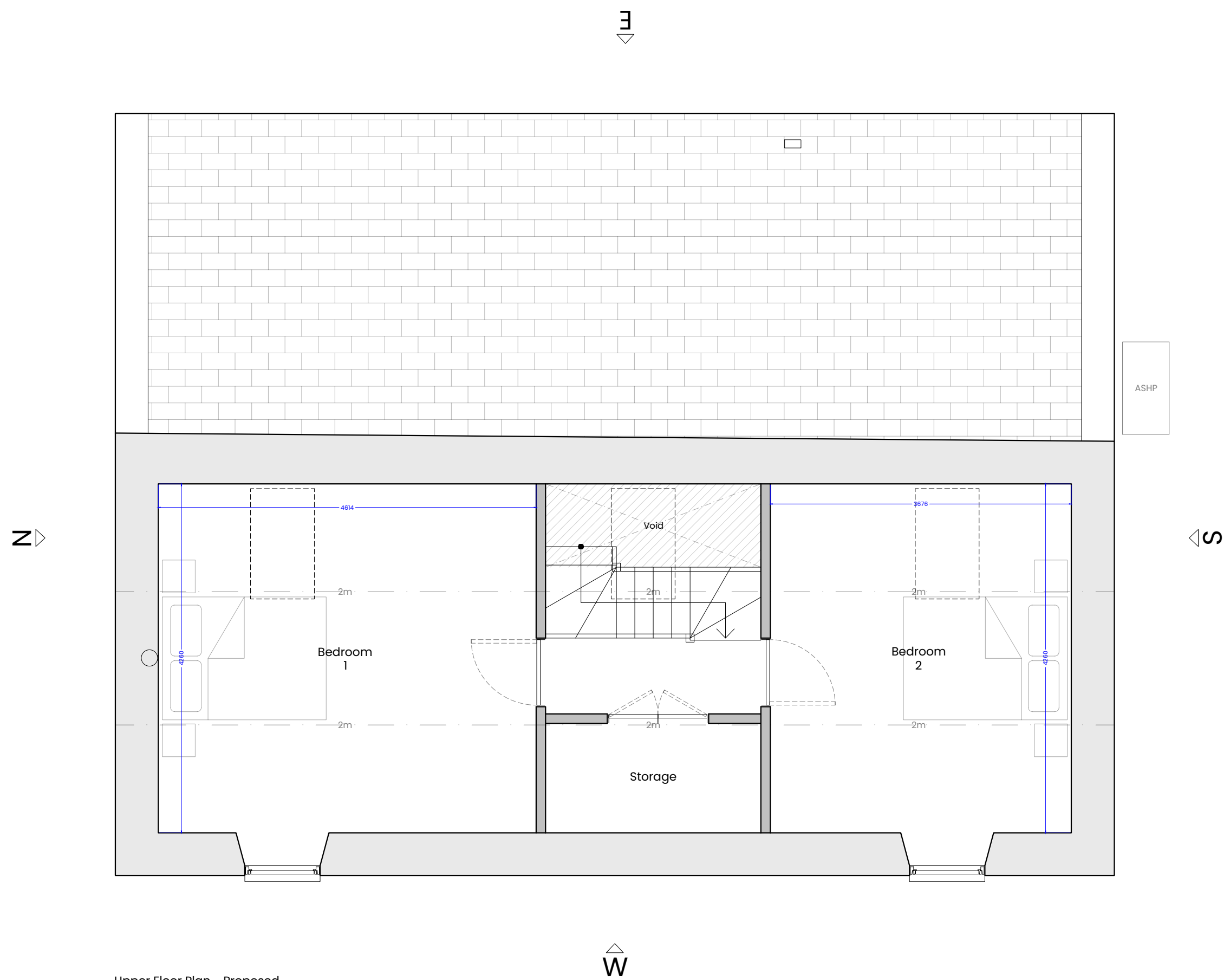
Upper Floor Plan - Proposed 1:50
