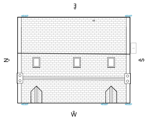
Roof Plan - Proposed 1:200
