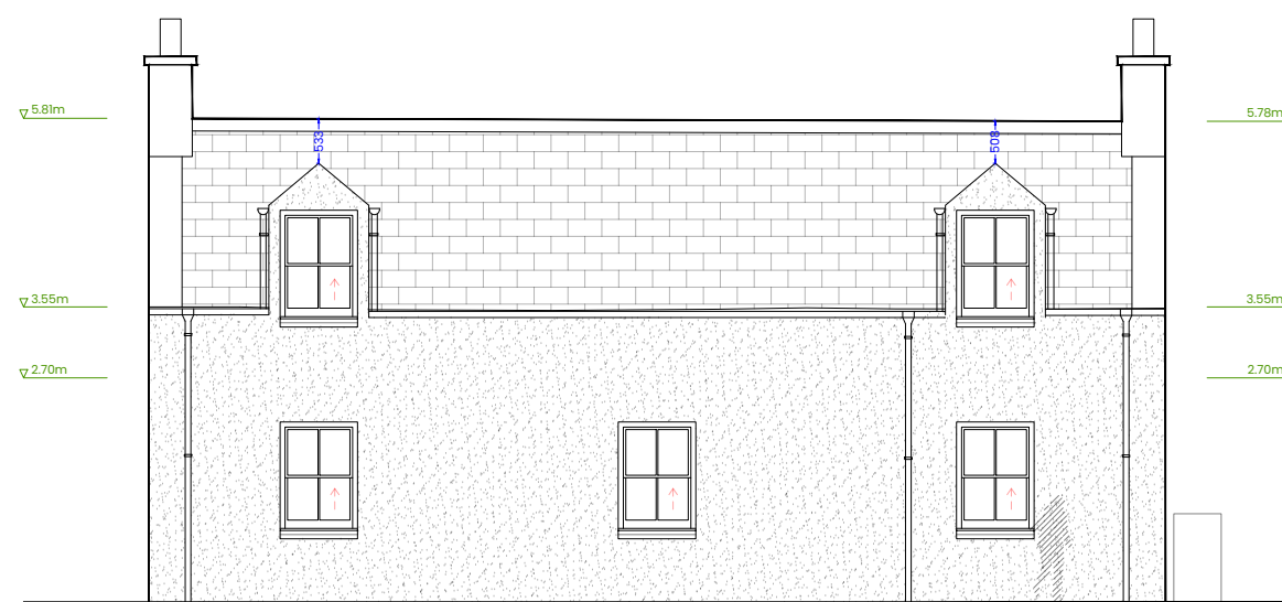
South Elevation - Proposed 1:100
