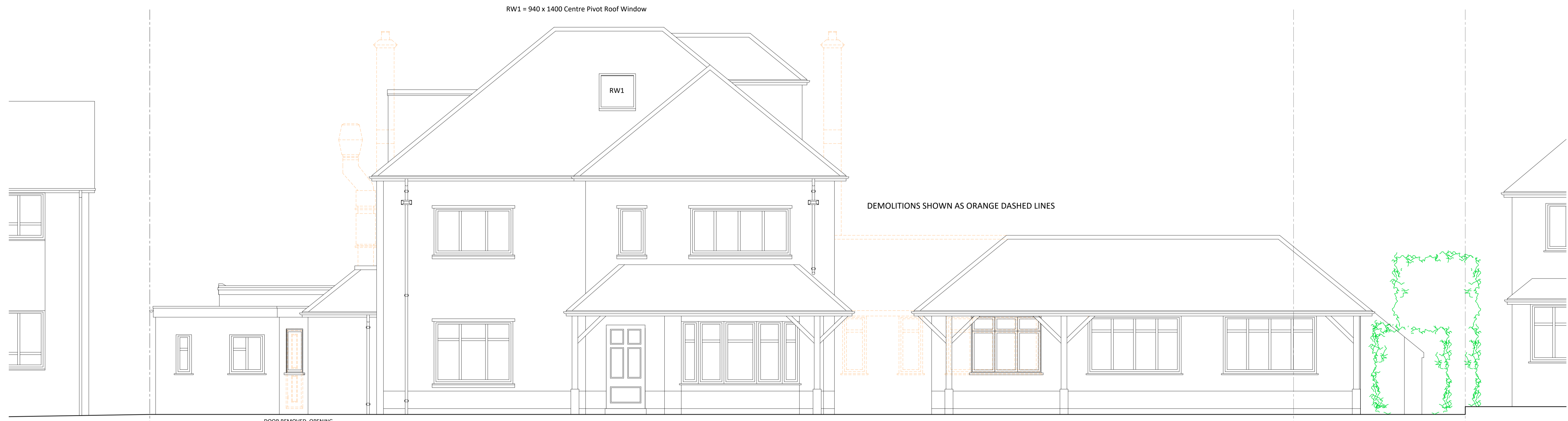
Proposed Front Elevation - South West 1:50 Scale
