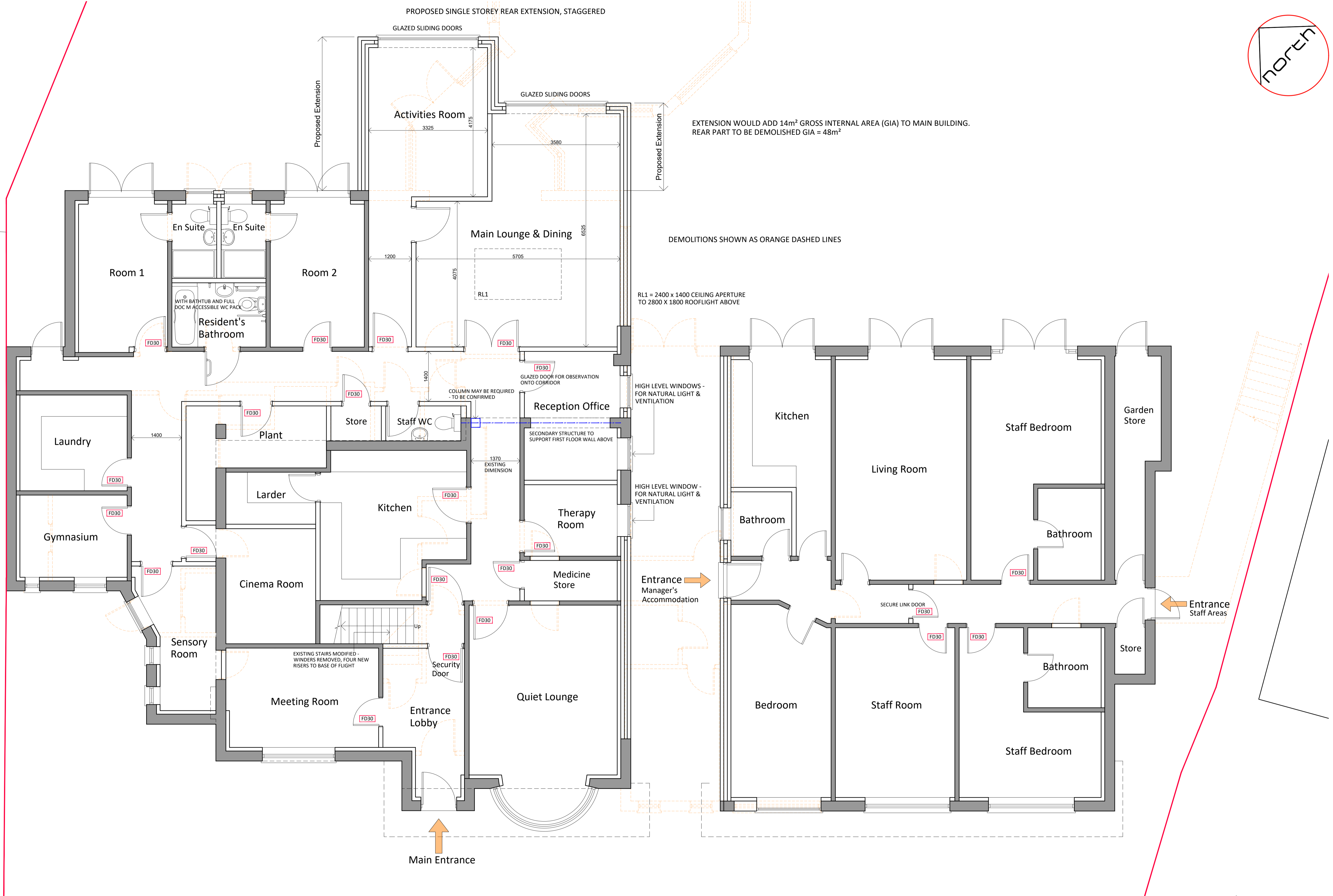
Proposed Ground Floor Plan 1:50 Scale
