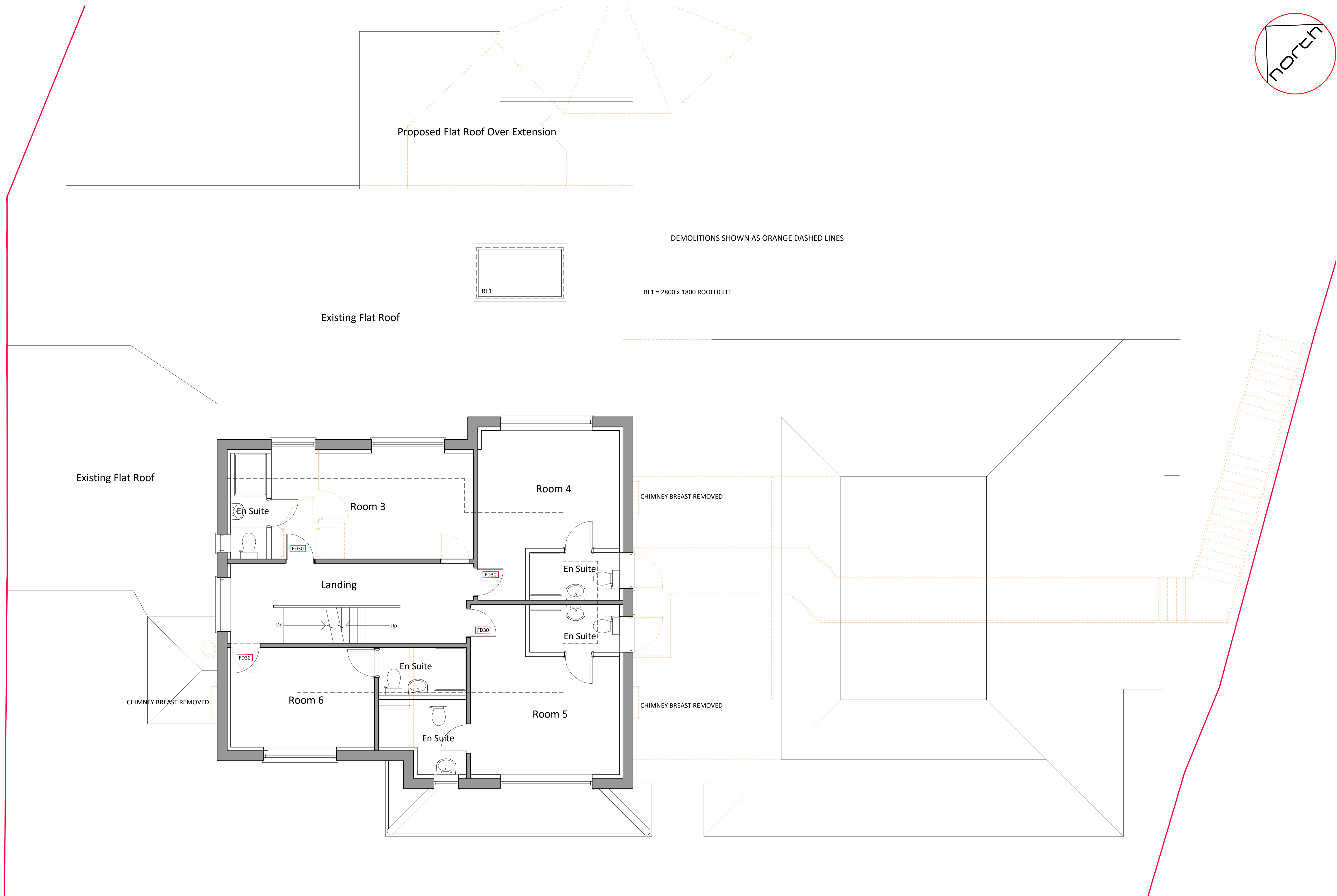
Proposed First Floor Plan 1:50 Scale
