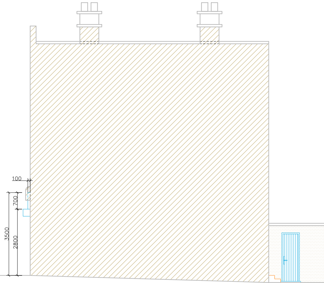
EXISTING SIDE ELEVATION-1
