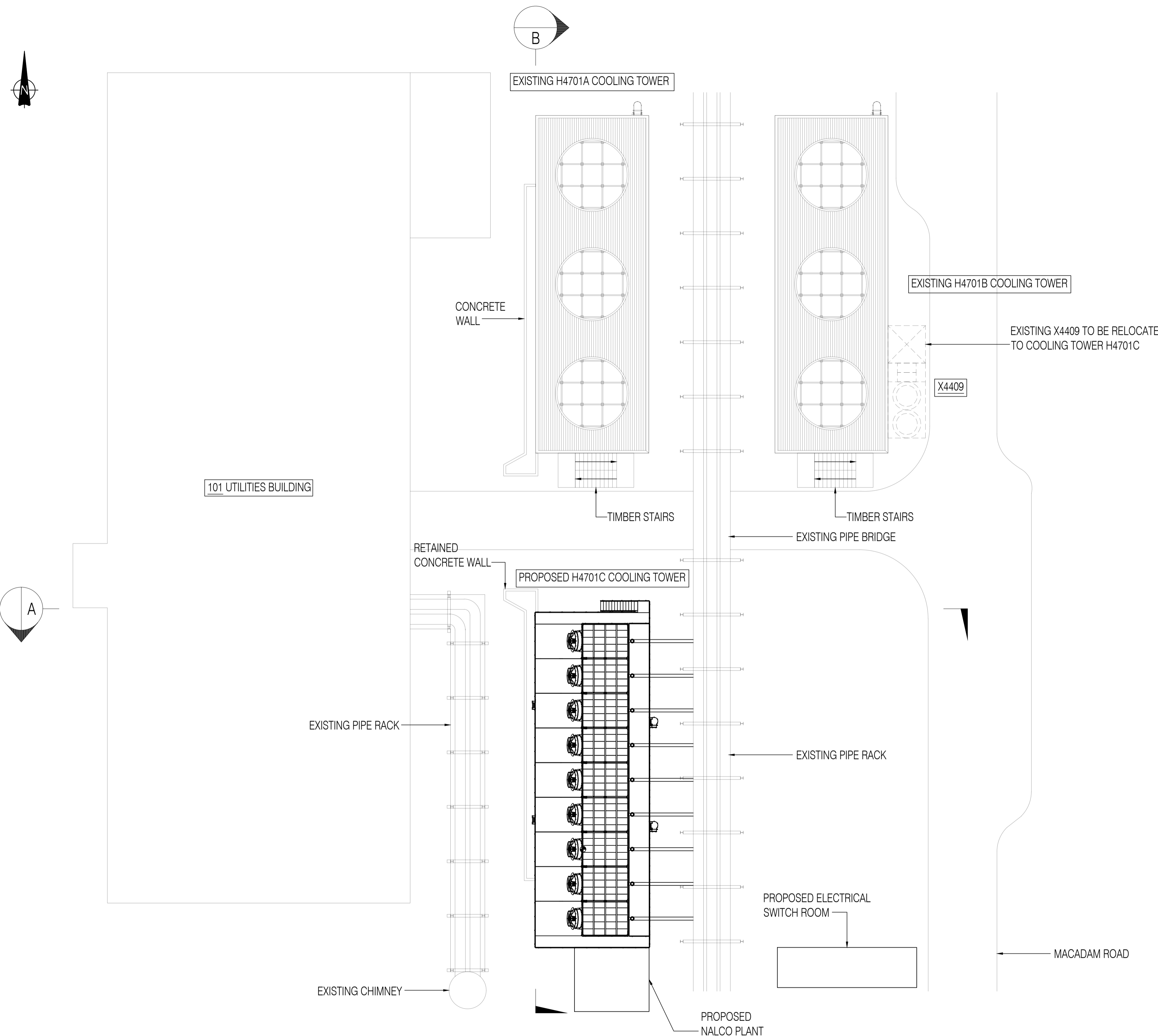
PLAN AS PROPOSED SCALE 1:200
