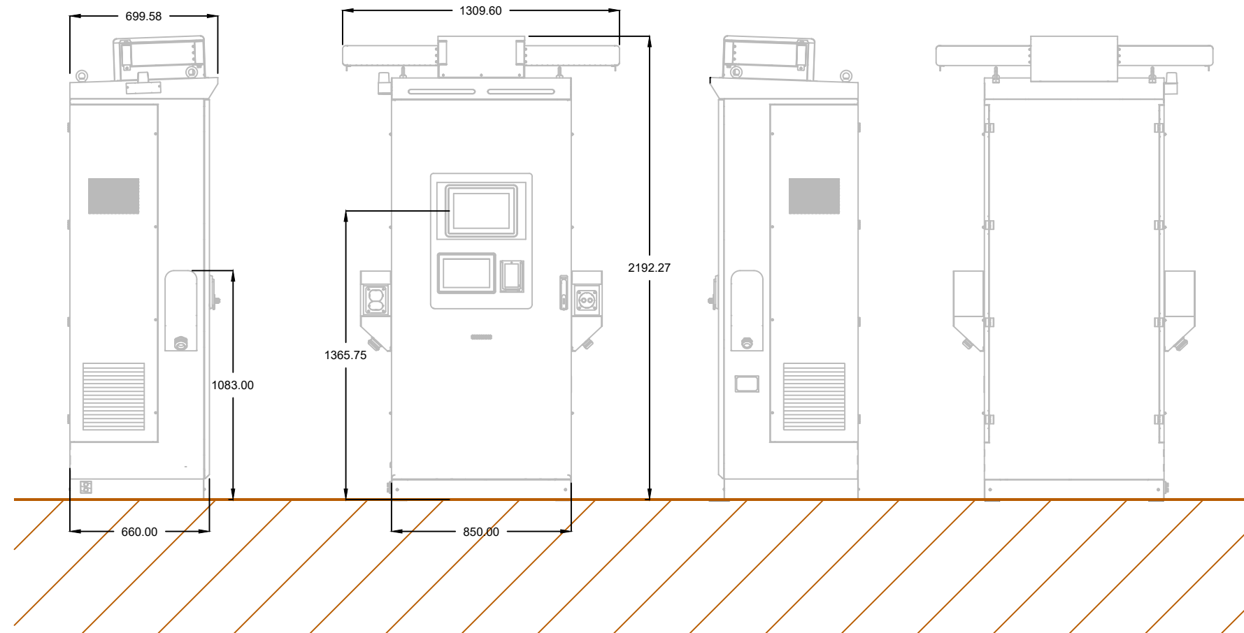
SIDE ELEVATION
