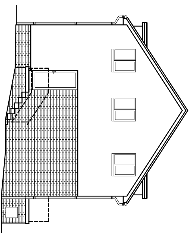
EXISTING SIDE ELEVATION 1:50
