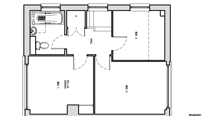
EXISTING FIRST FLOOR PLAN 1:50
