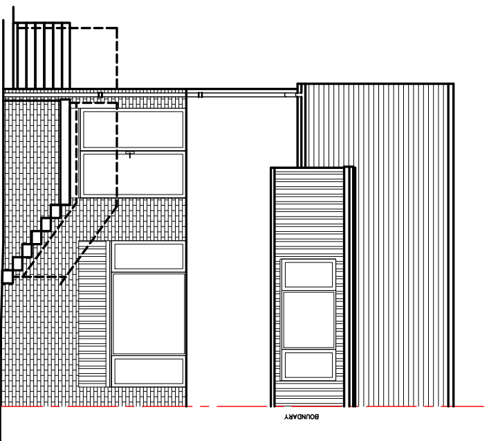
EXISTING FRONT ELEVATION 1:50
