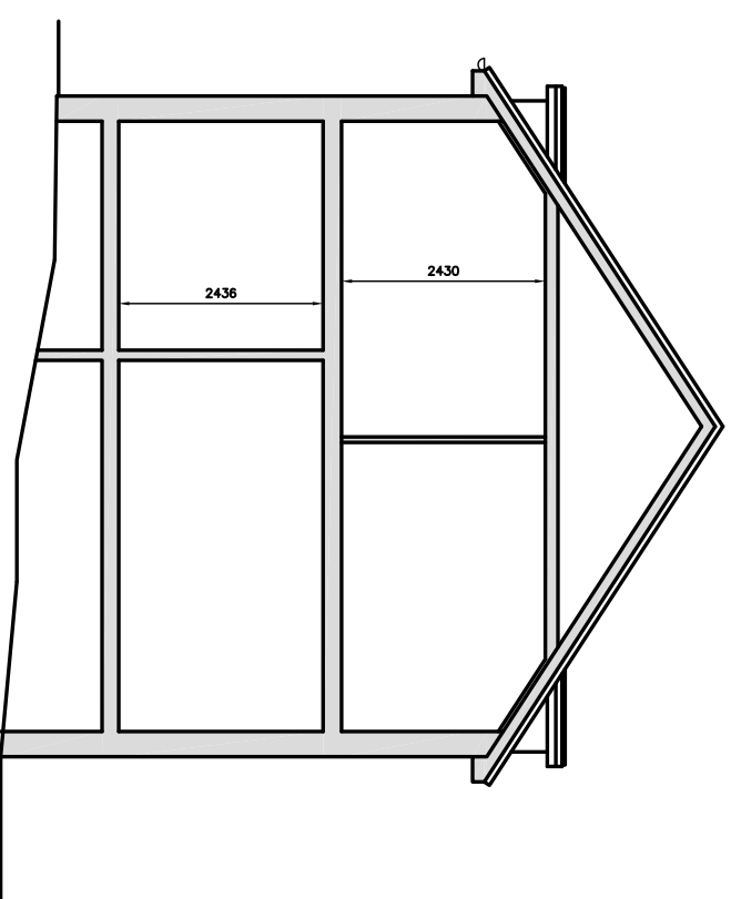
EXISTING SECTION 1:50
