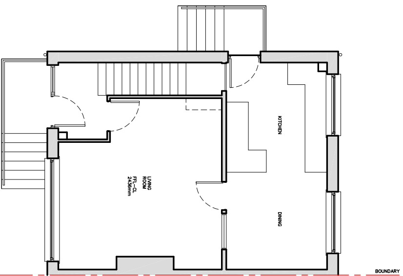
EXISTING GROUND FLOOR PLAN 1:50
