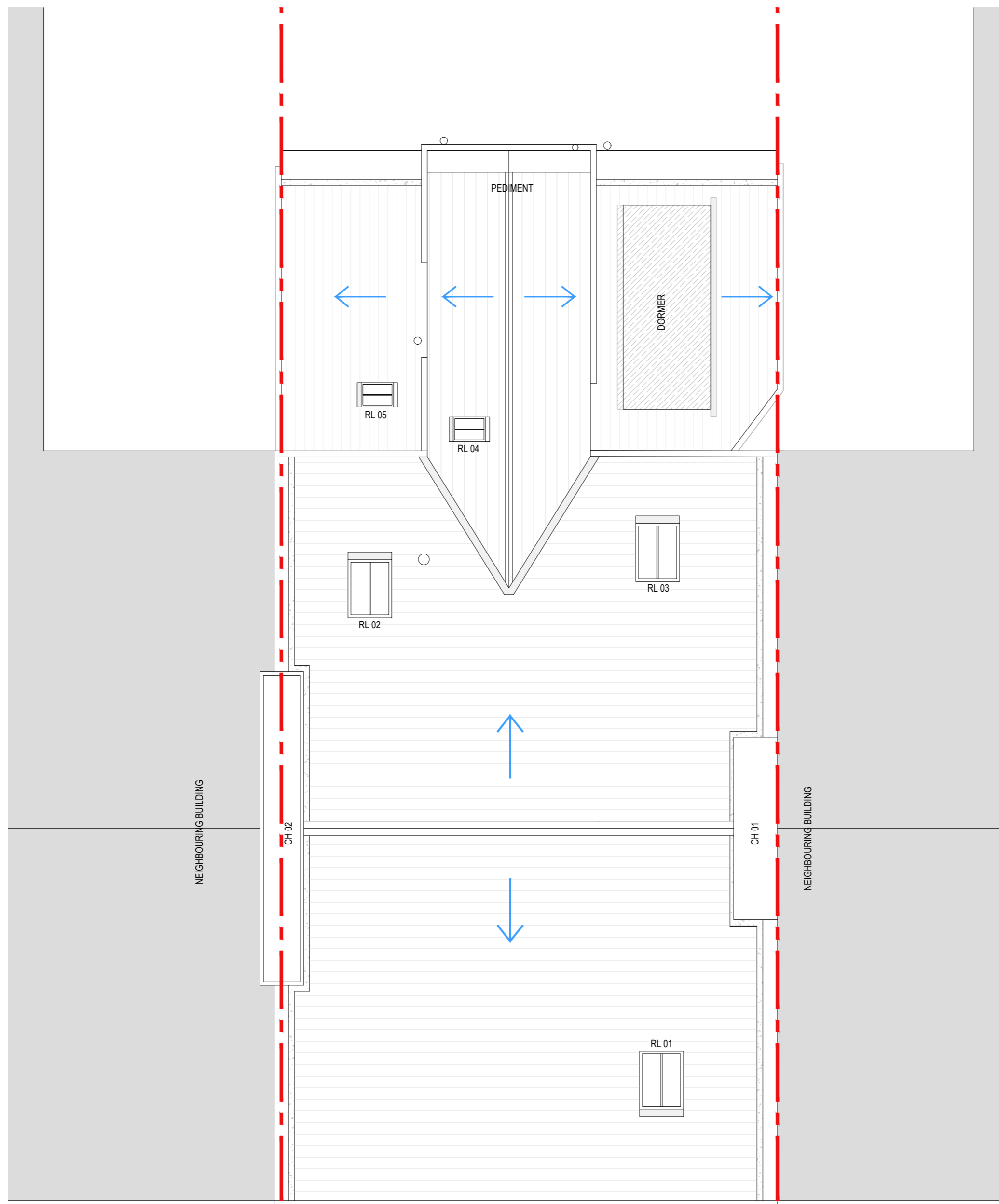
EXISTING ROOF PLAN
