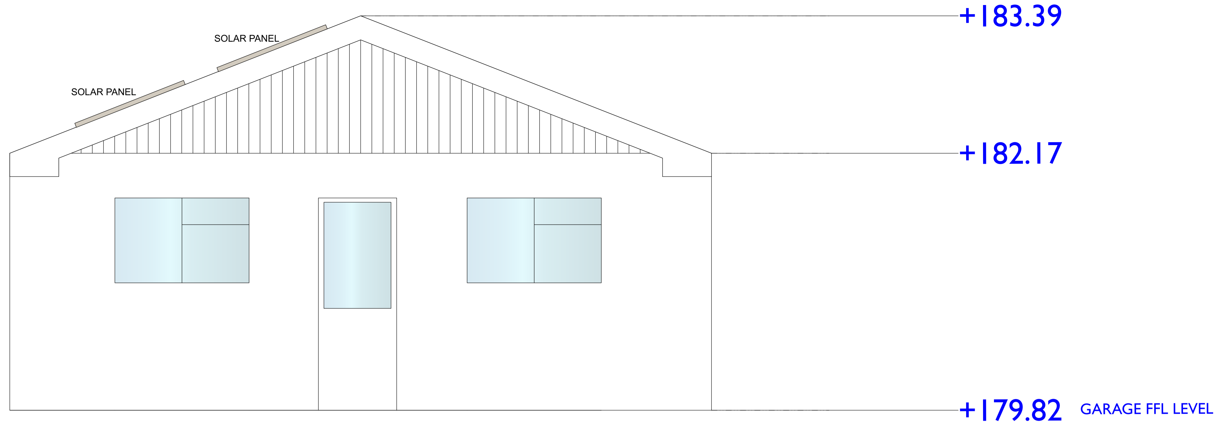
BACK PROPOSED GARAGE ELEVATION
