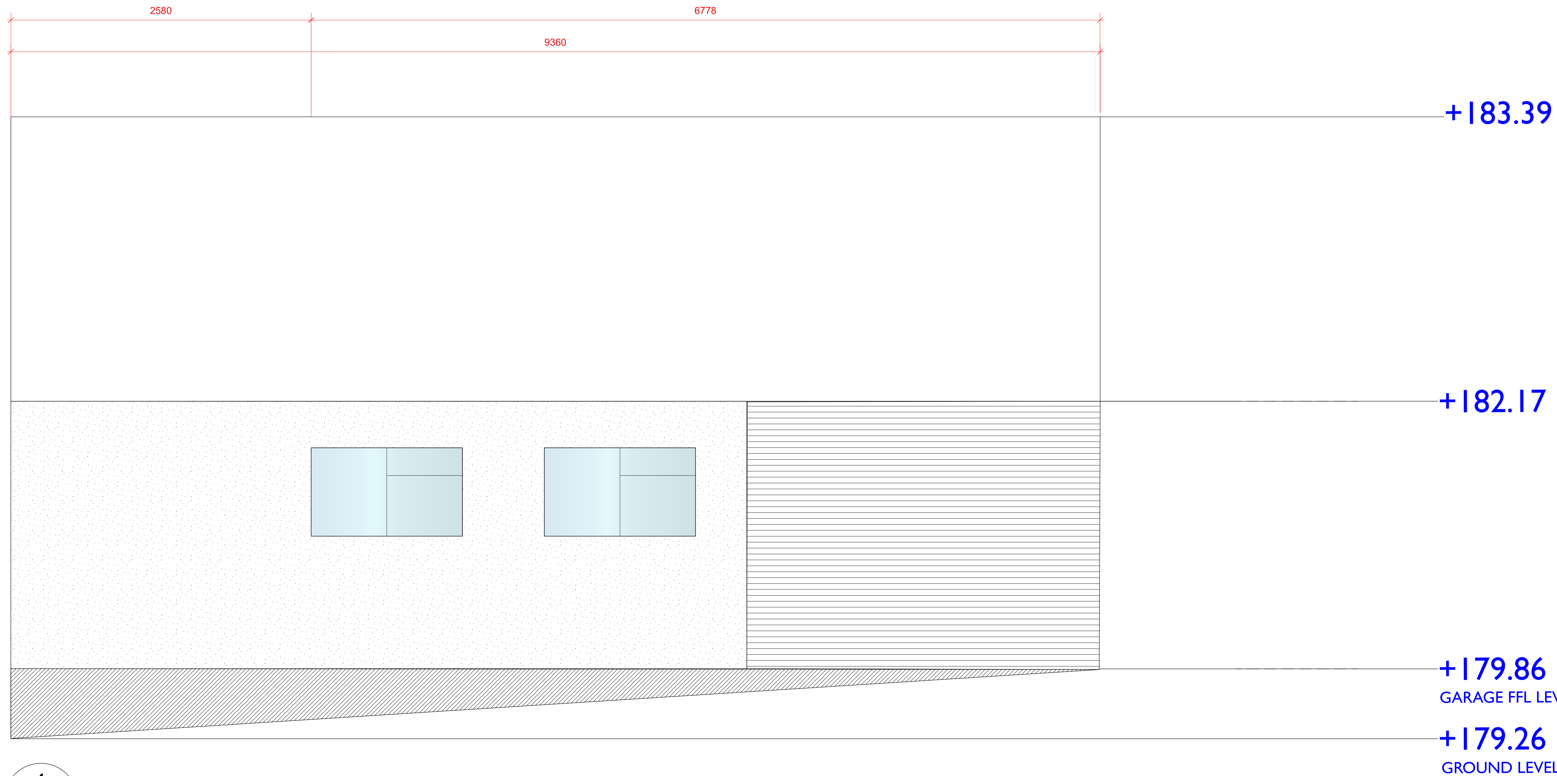
LEFT SIDE PROPOSED ELEVATION
