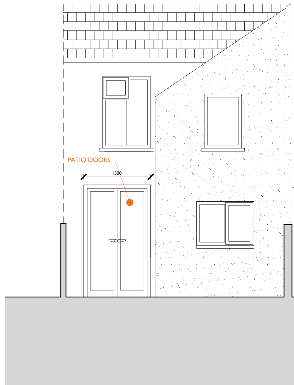
+EL Proposed Rear Elevation - scale 1:50 at A3
