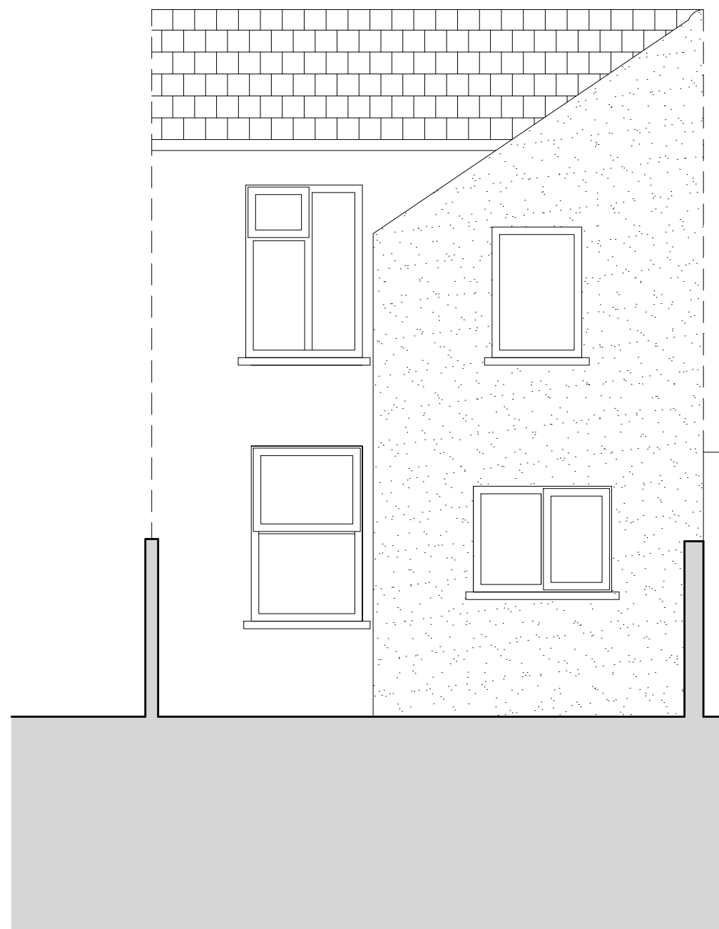
+EL Existing Rear Elevation - scale 1:50 at A3
