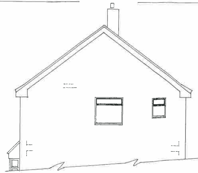
SIDE [WEST] ELEVATION
