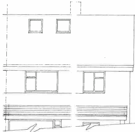
FRONT [NORTH] ELEVATION
