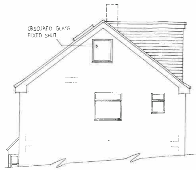
SIDE [WEST] ELEVATION
