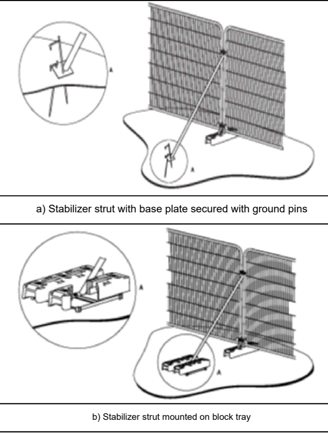
Images taken from British Standard 5837:2012 - Trees in relation to design, demolition and construction - Recommendations
