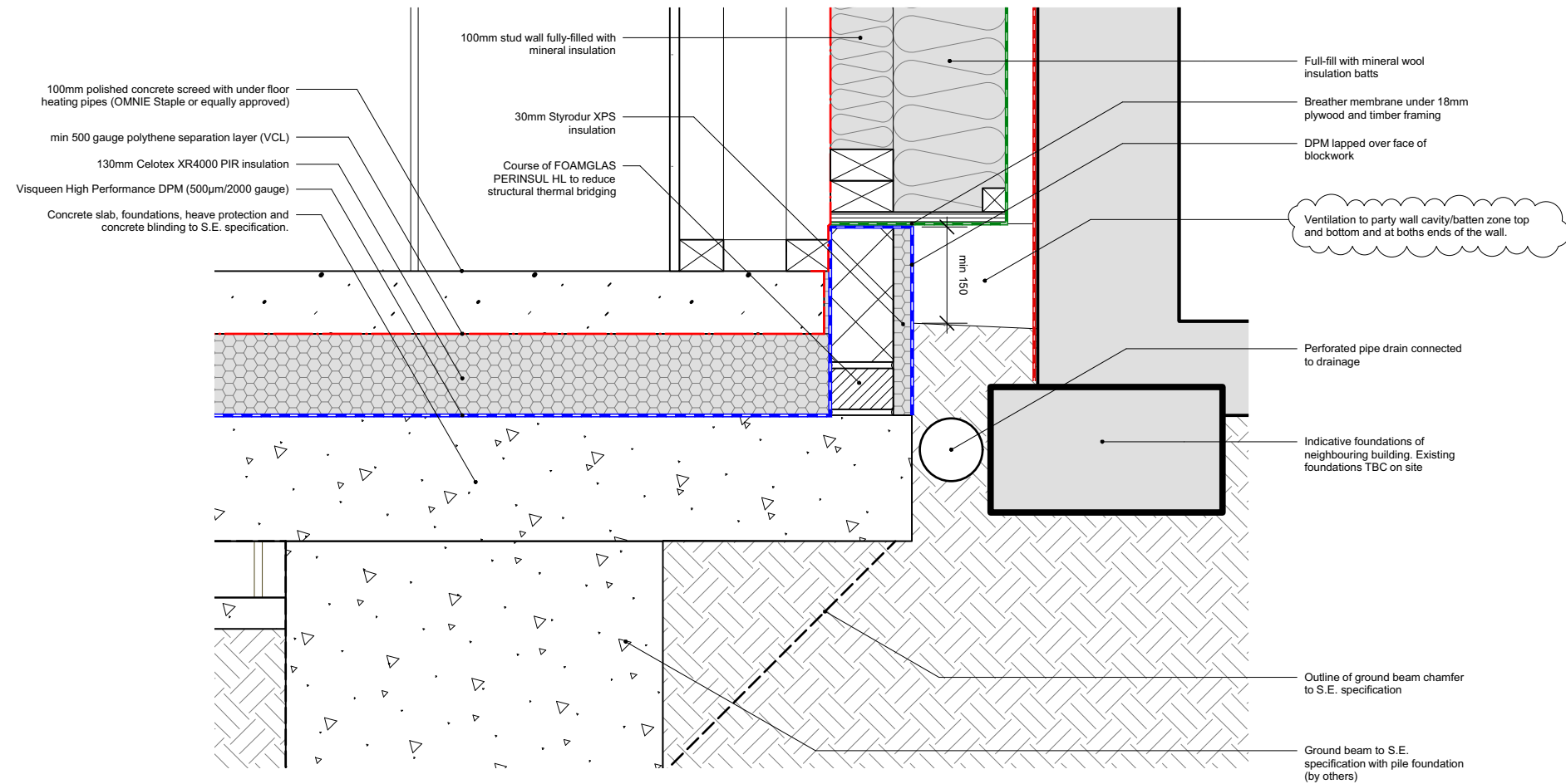
01 Party wall, foundation & flat roof eaves detail 1:10 @ A3
