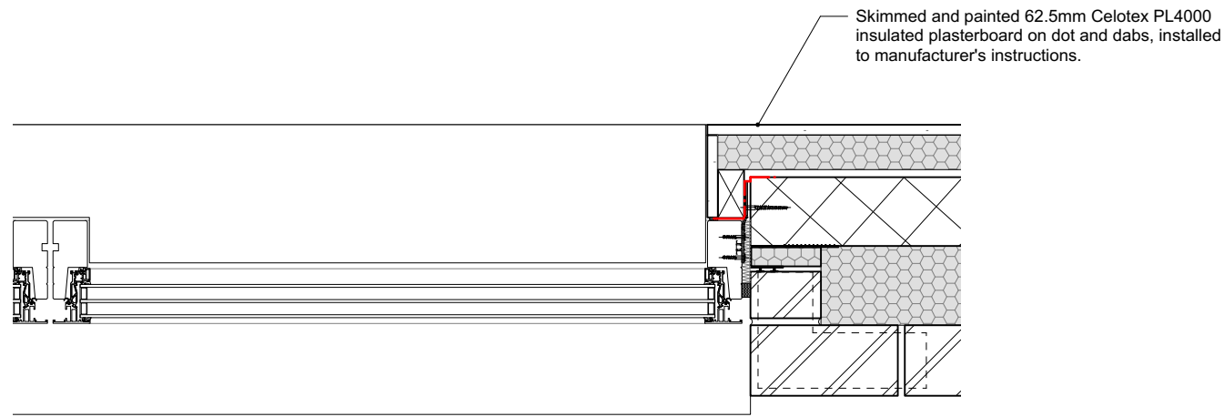
01 Master bedroom window jamb detail 1:10 @ A3
