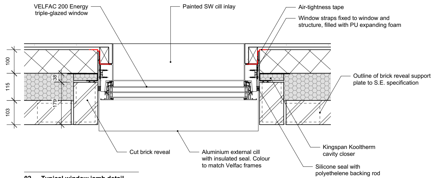
02 Typical window jamb detail 1:10 @ A3
