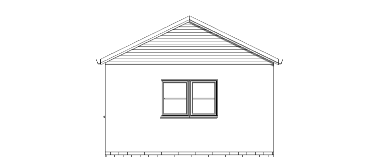
4 Rear Elevation (North) 1 : 100
