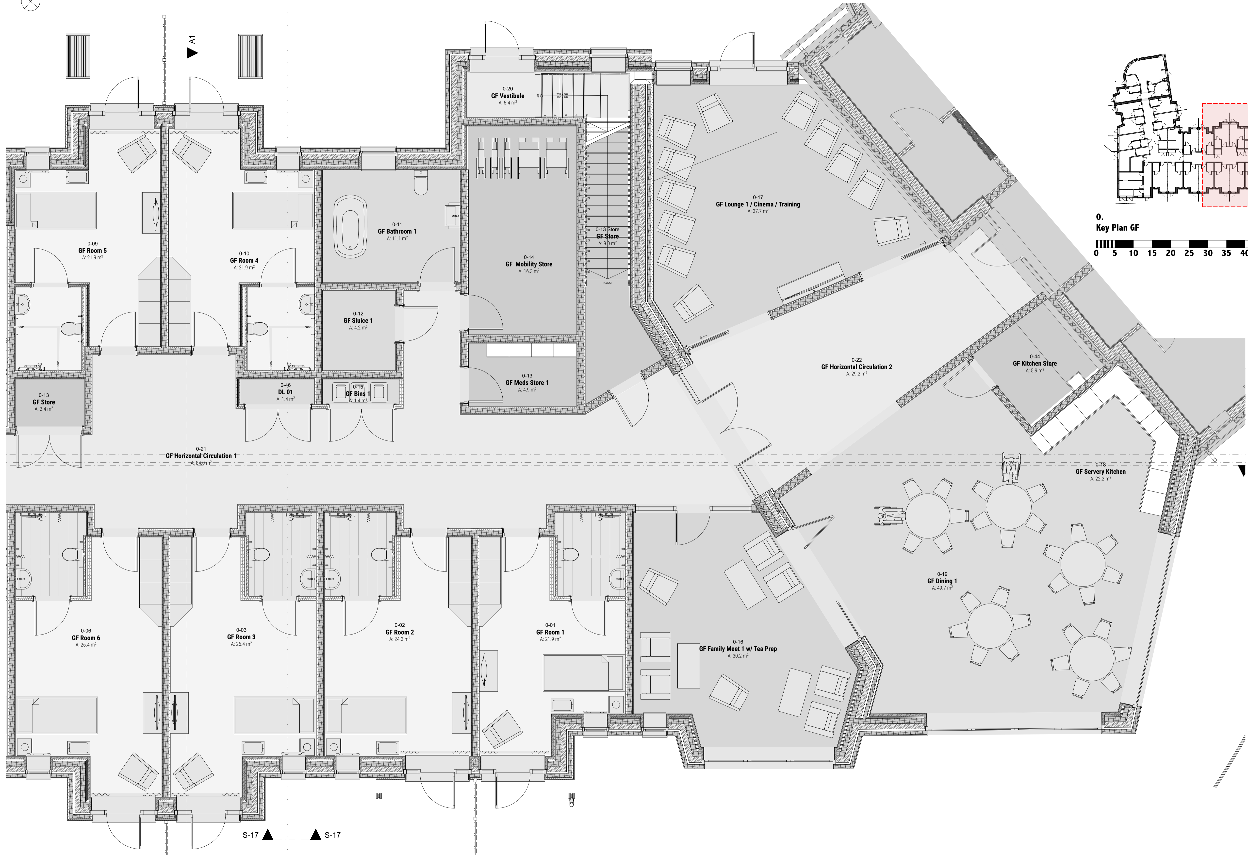
0. Ground South 1:50 0 5
