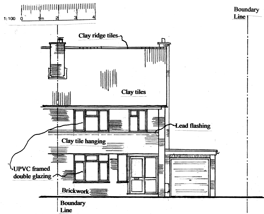
FRONT ELEVATION
