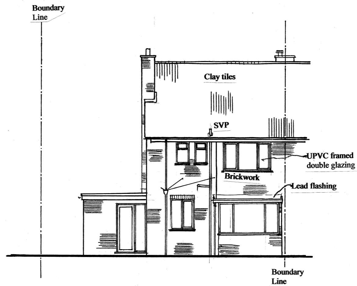
REAR ELEVATION
