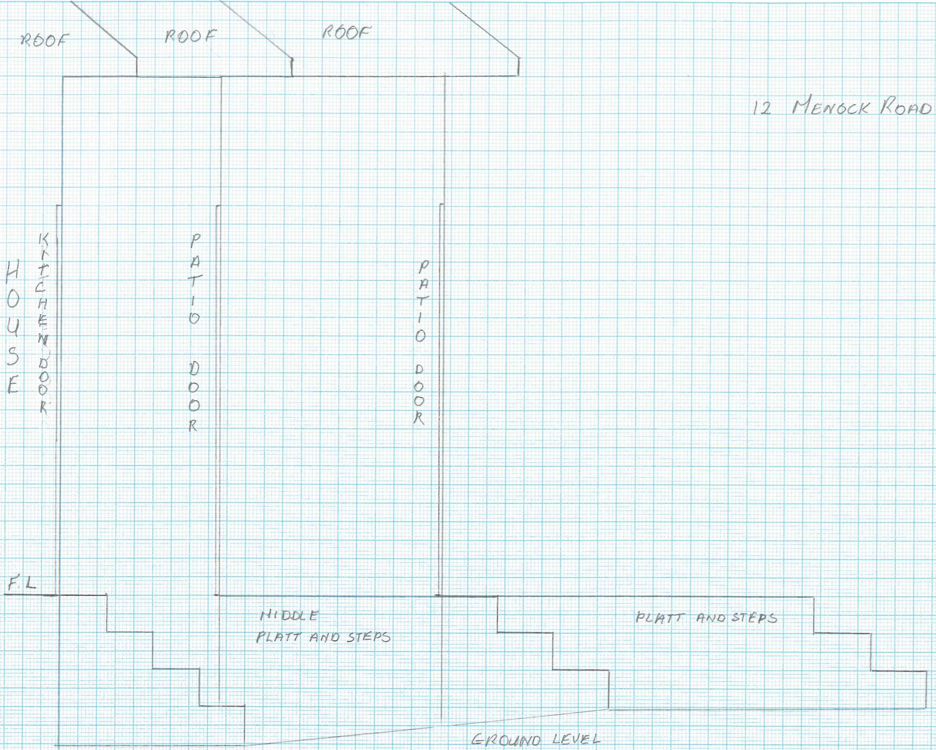
SECTION WEST ELEVATION AS EXISTING SCALE 1:20
