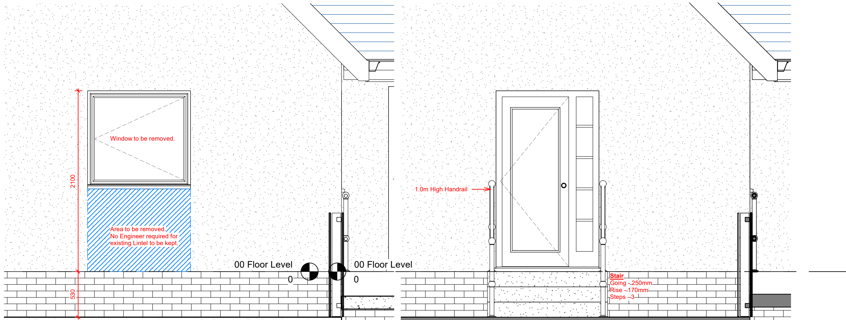
1 Existing Detail Elevation 1:25
