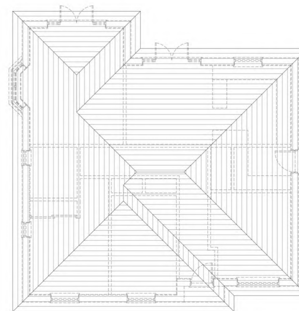
Roof Plan
