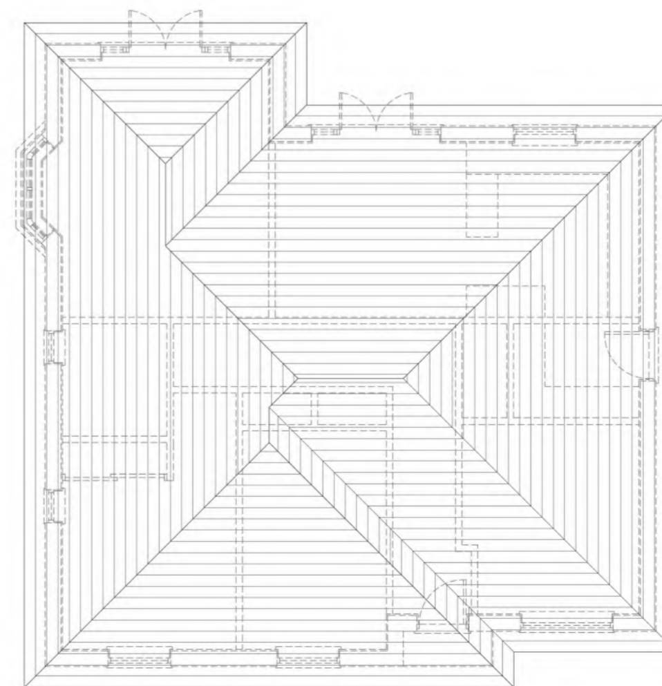
Roof Plan
