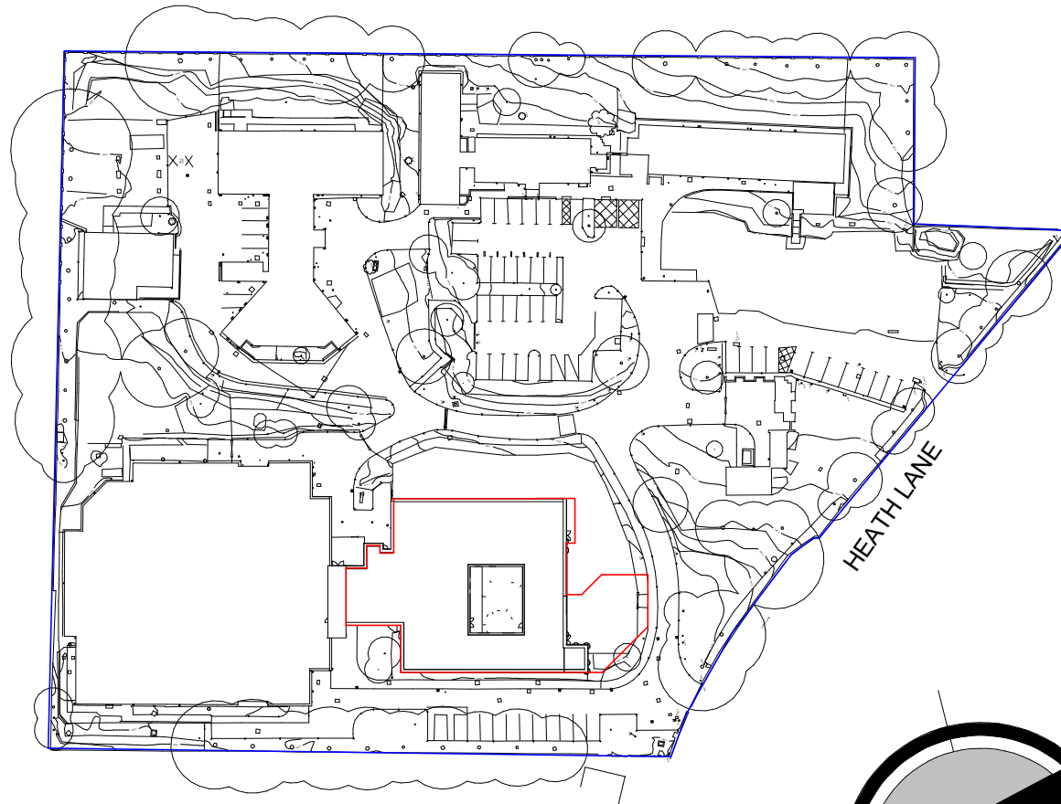
1 Site Location Plan 1 : 1250
