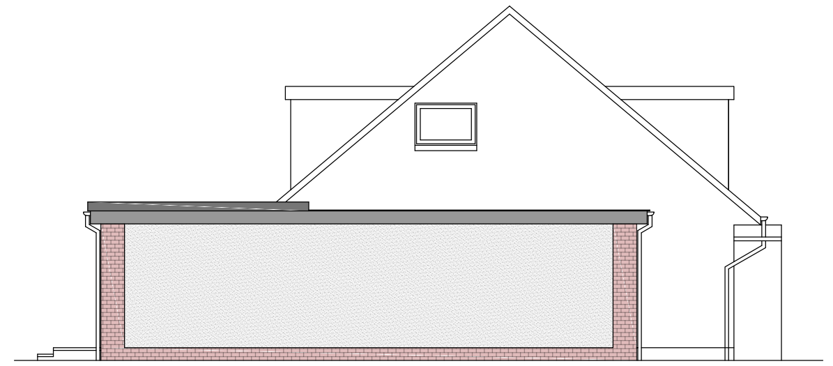
Proposed Side Elevations (scale 1:100)
