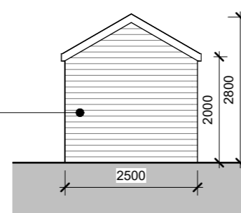
Proposed North Elevation 1 : 100
