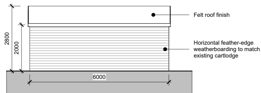
Proposed West Elevation 1 : 100
