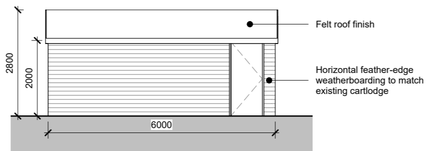
Proposed East Elevation 1 : 100
