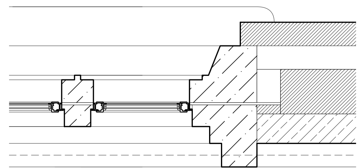
Ground Floor - Detail 1
