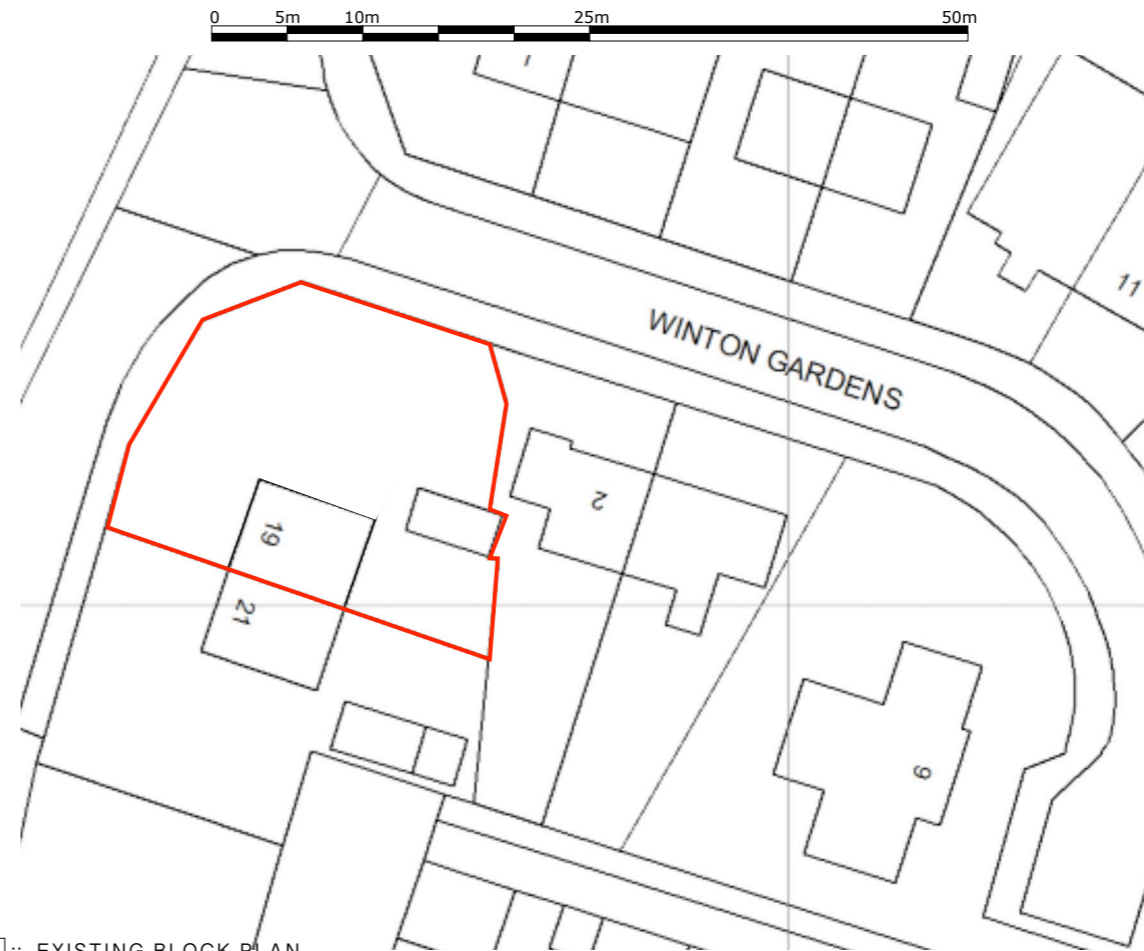
P :: EXISTING BLOCK PLAN 22 scale: 1:500
