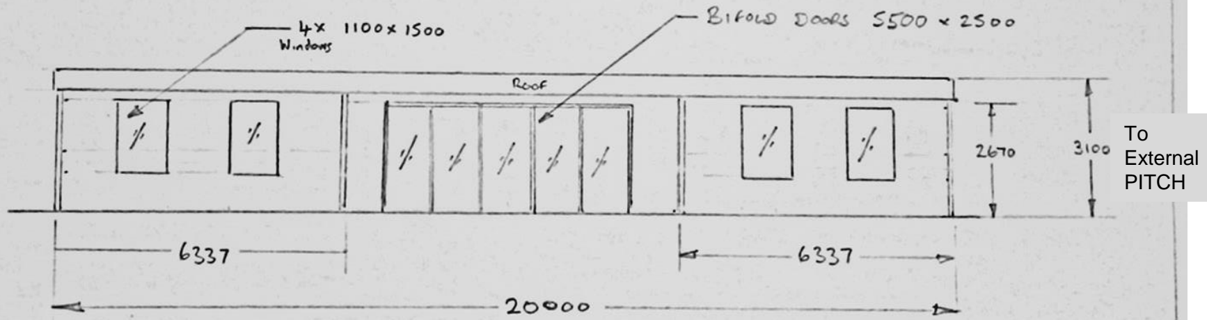
BERLLAN - DDU | FRONT ELEVATION | SCALE 1:100
