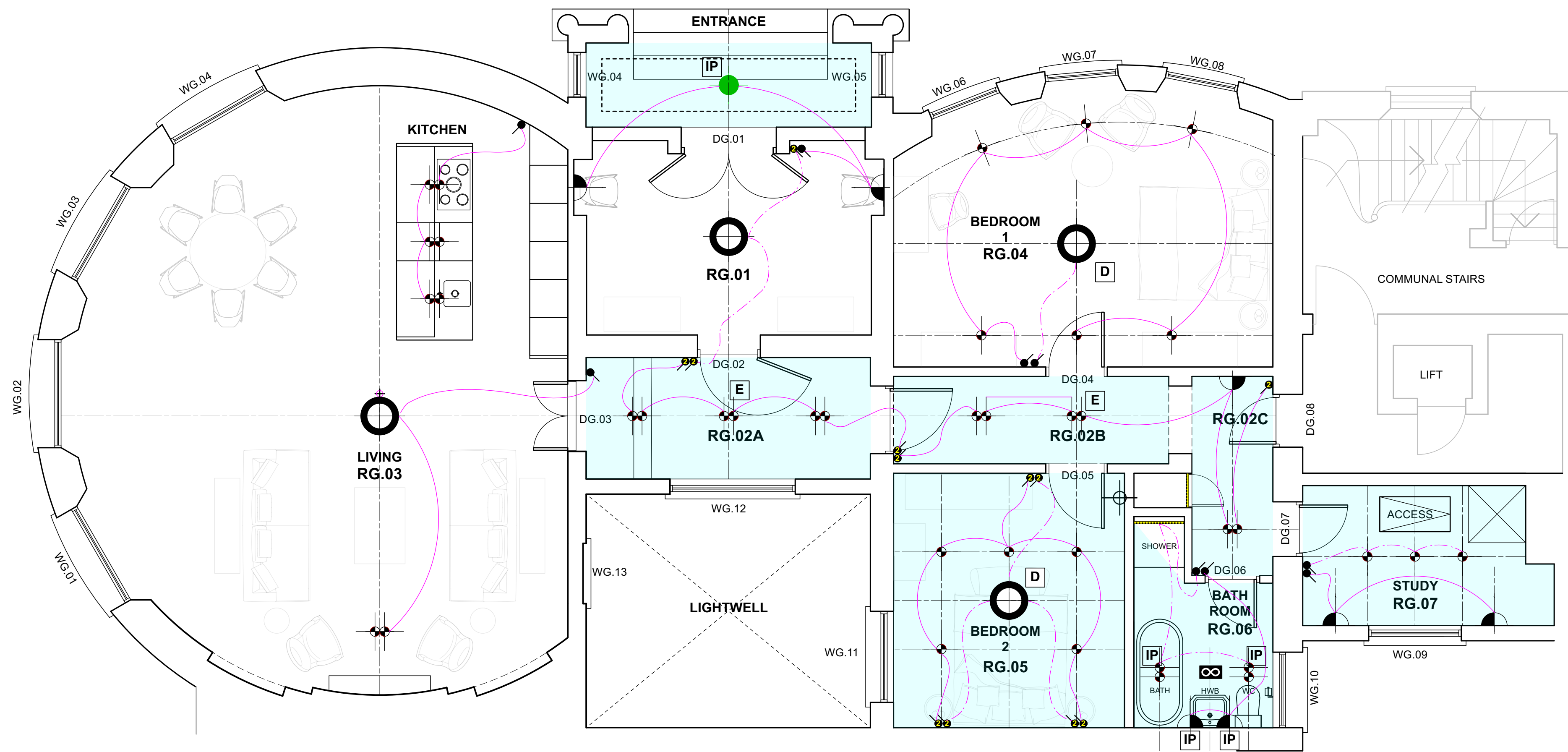
PROPOSED RCP GROUND FLOOR PLAN
