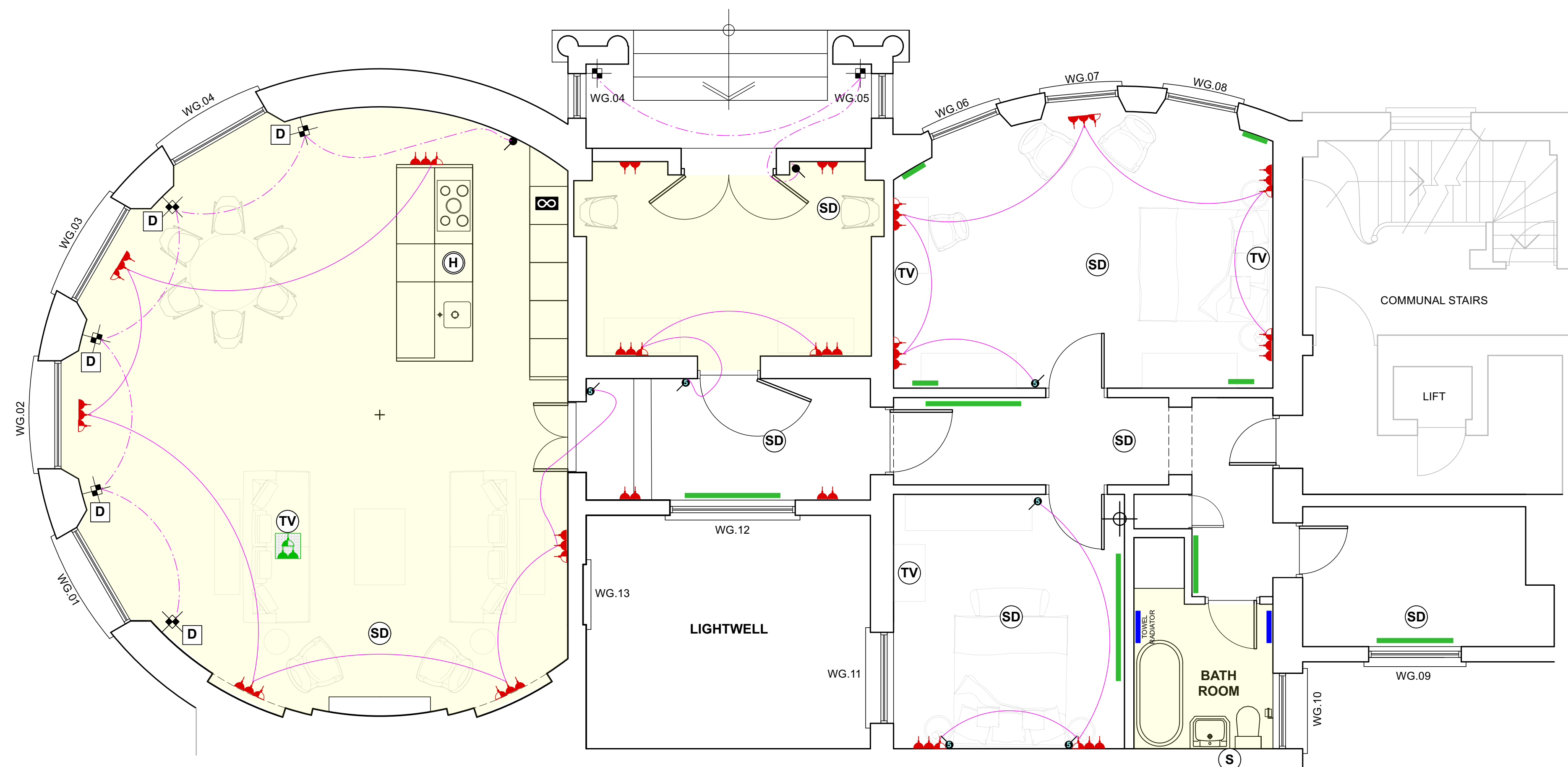
PROPOSED GROUND FLOOR LOW LEVEL POWER PLAN
