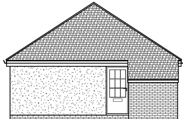
EXISTING RIGHT SIDE ELEVATION
