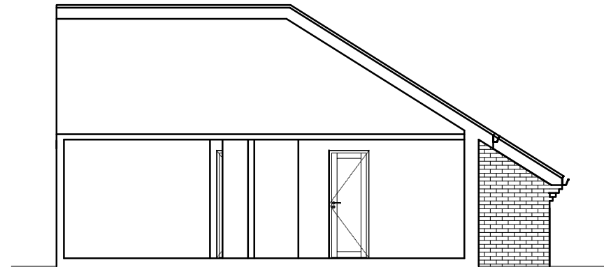
EXISTING SECTION
