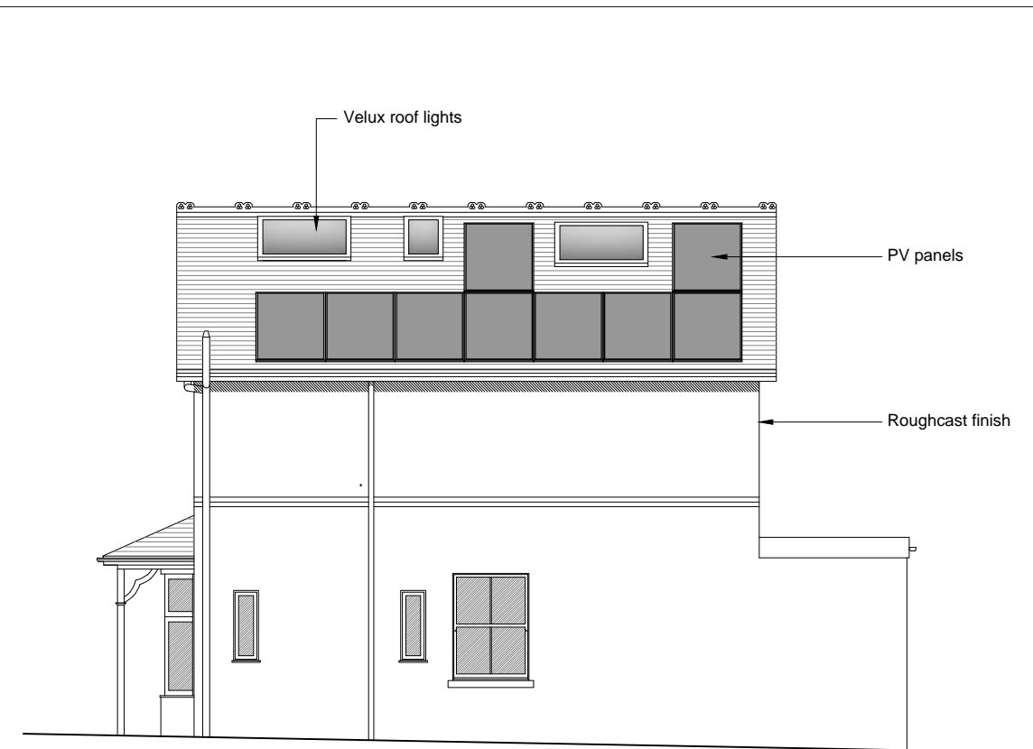
West Elevation
