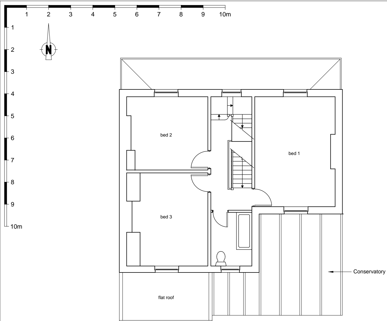
1 - First floor plan existing
