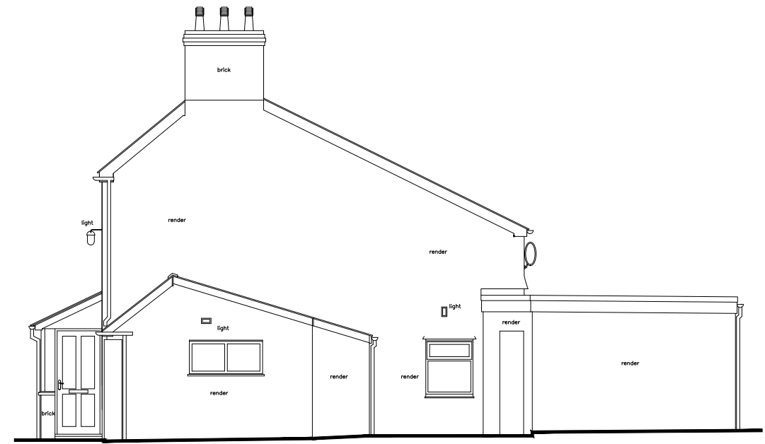
Existing Side Elevation (West)
