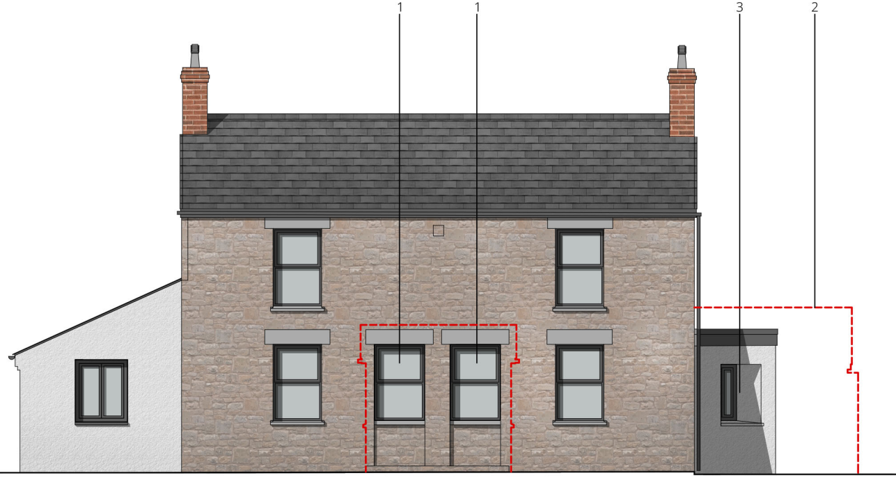
| Front Elevation
