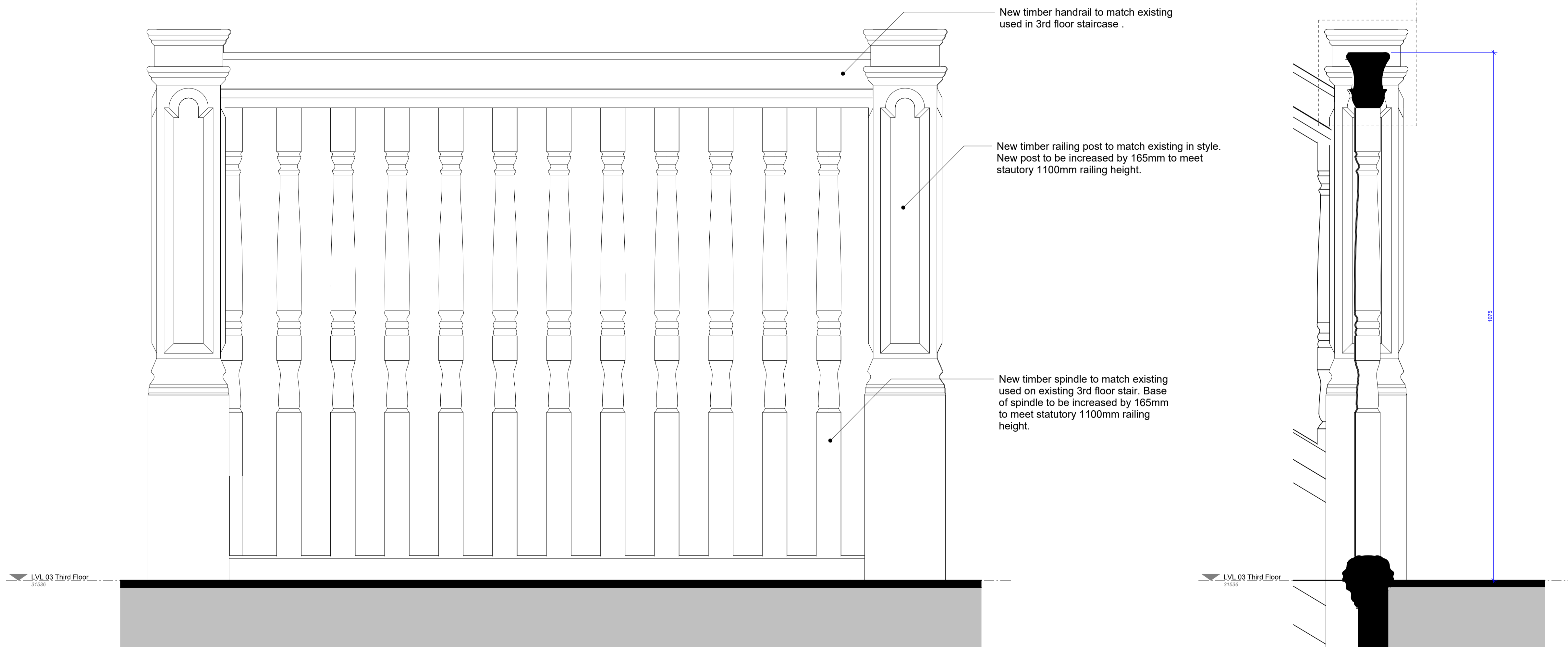
1 LVL 03 - Baluster Elevation 1:5
