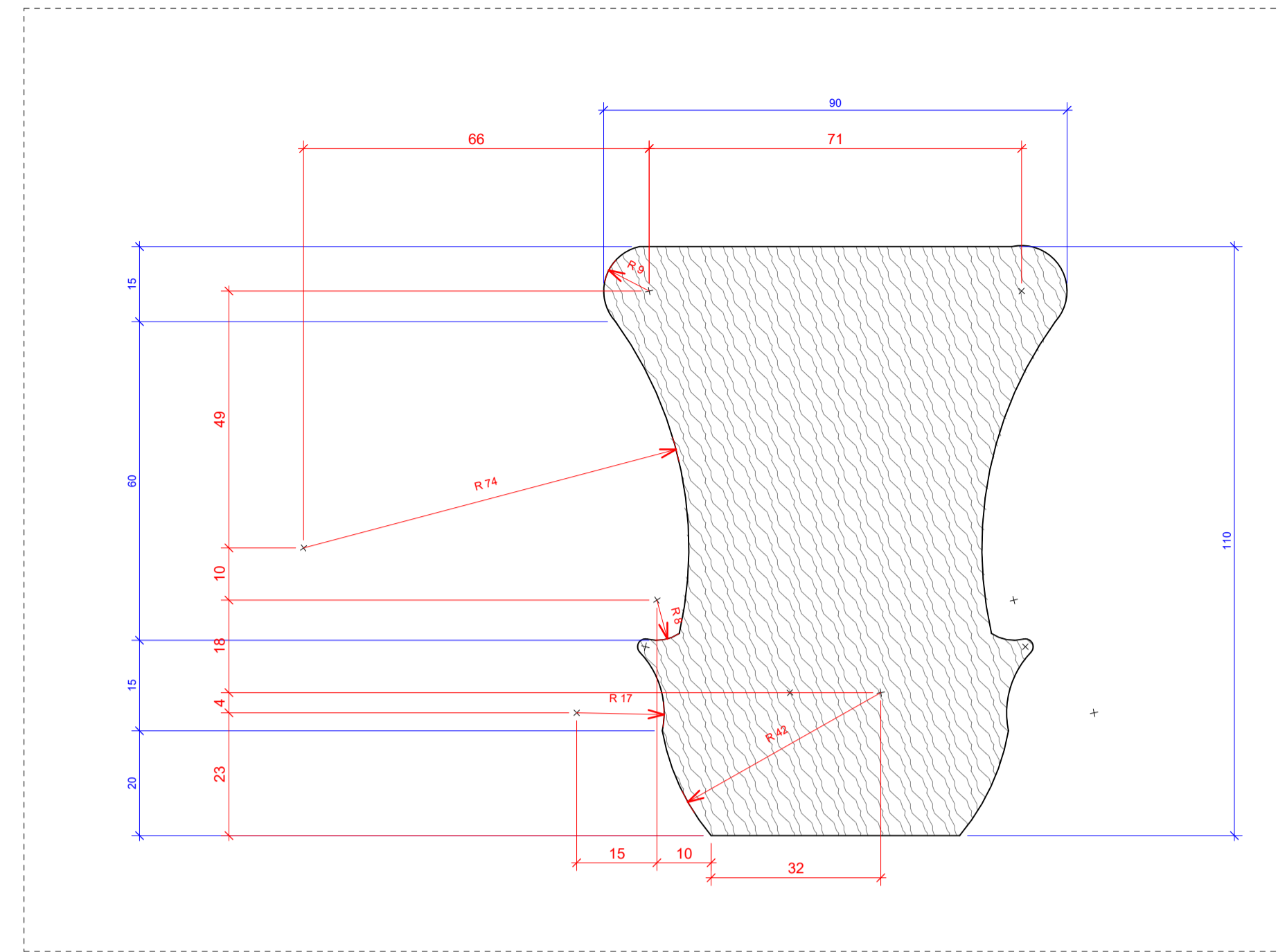
3 LVL 03 - Handrail Profile 2 1:1
